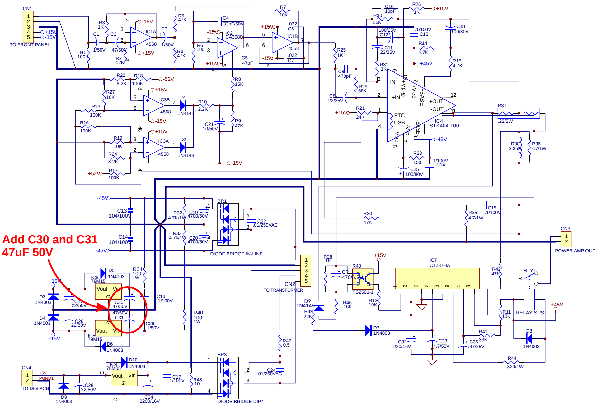
PROFILE POWER SCHEMATIC
