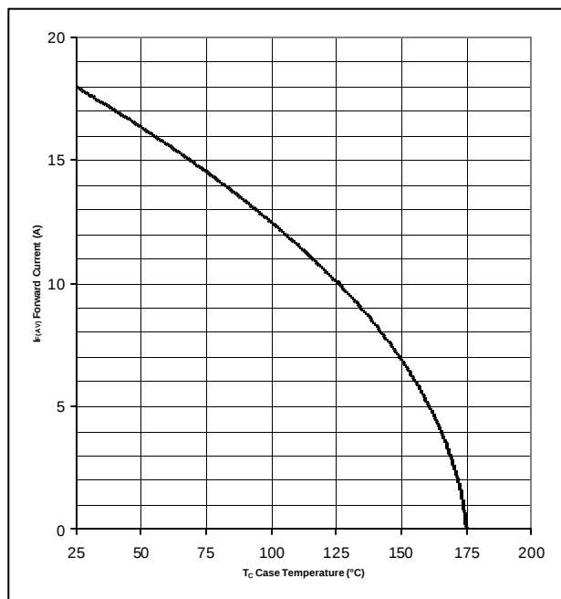
Figure 3. Current Derating
