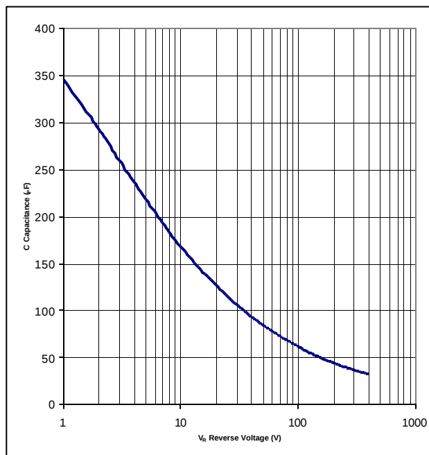
Figure 4. Capacitance vs. Reverse Voltage
