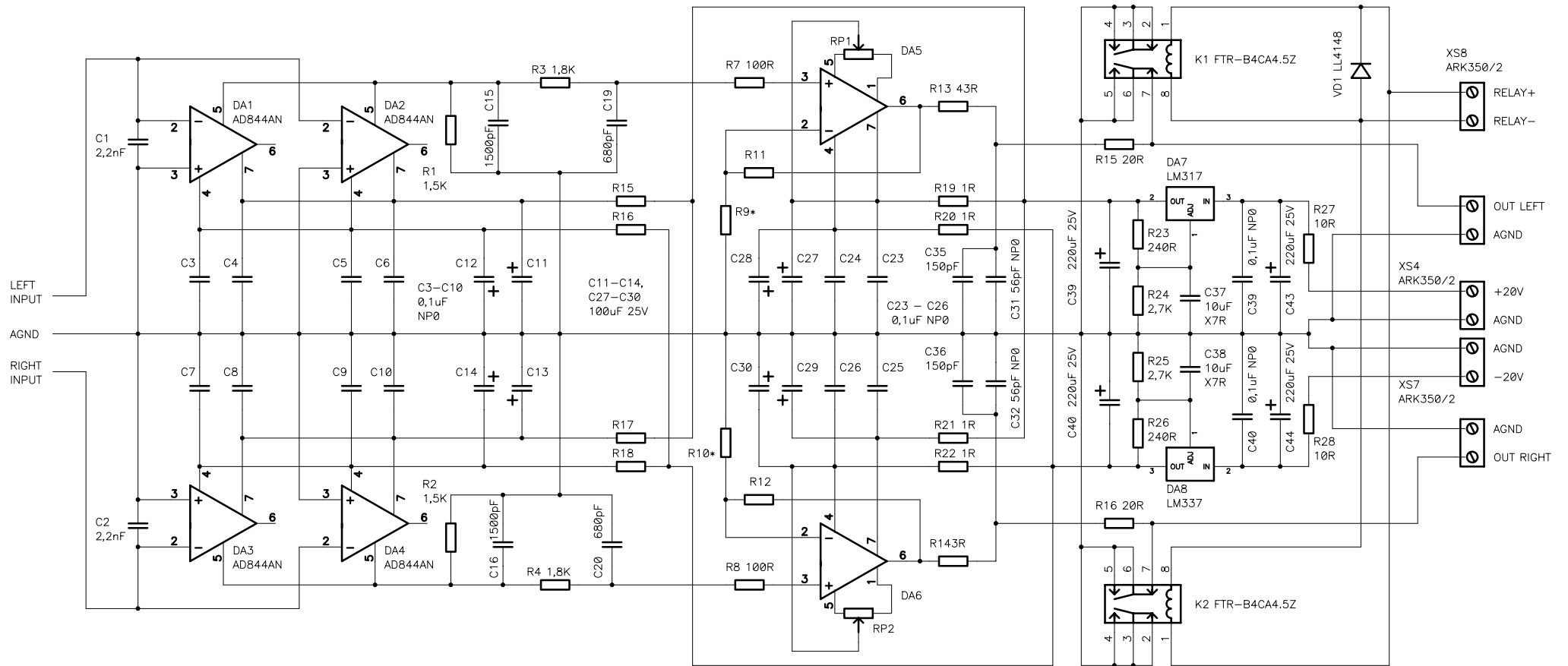
DAC Analog Stage V4.2 "Peter Gunn"
