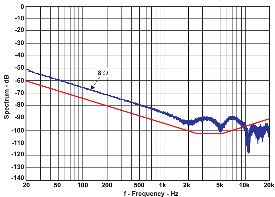
Figure 18. Pop/Click (BTL)
