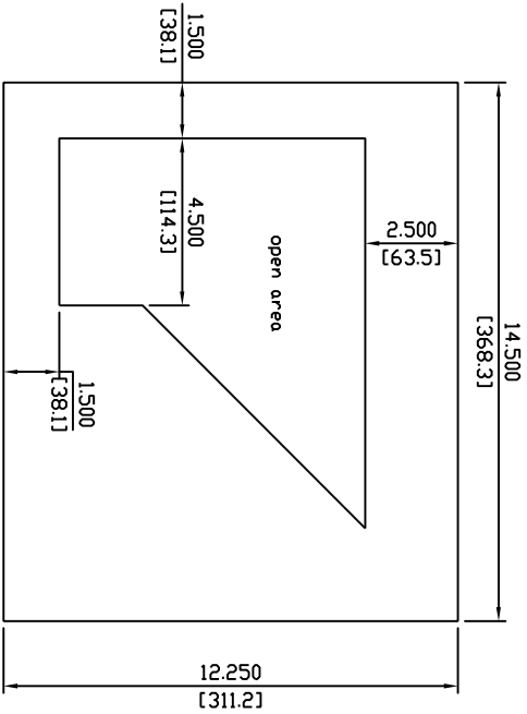
Detail upper shelf brace
