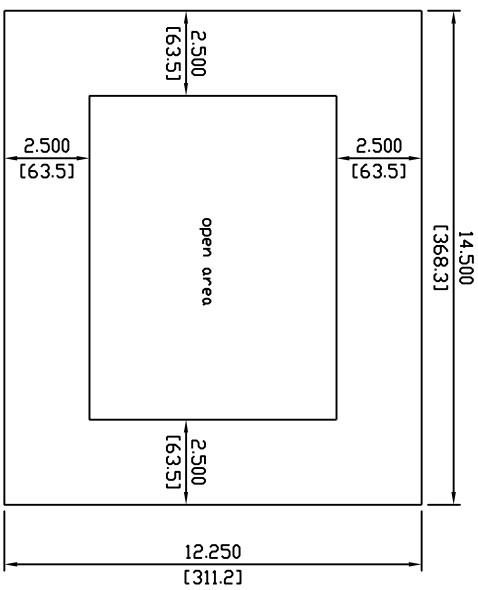
Detail lower shelf brace
