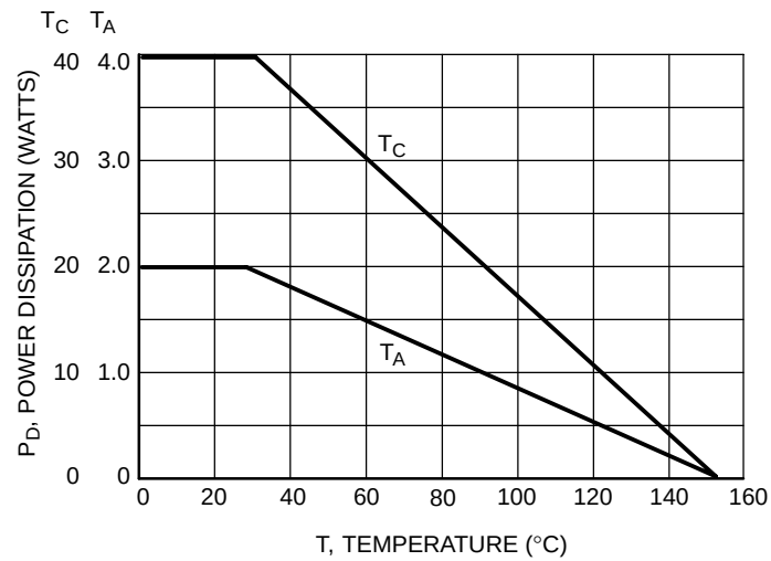
Figure 1. Power Derating
