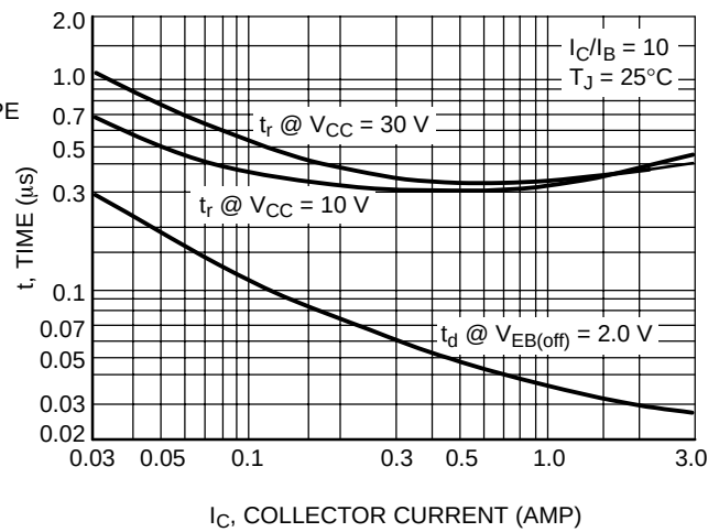
Figure 3. Turn-On Time
