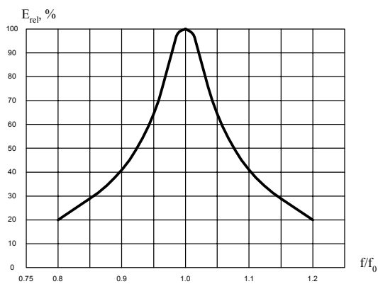
Figure 1 – Dependence of sensitivity as function of normalized frequency, T_{amb} = 25^{\circ}C (amplitude-frequency response).
