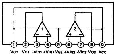
IC2 : \mu PC4570HA Dual OP-Amp
