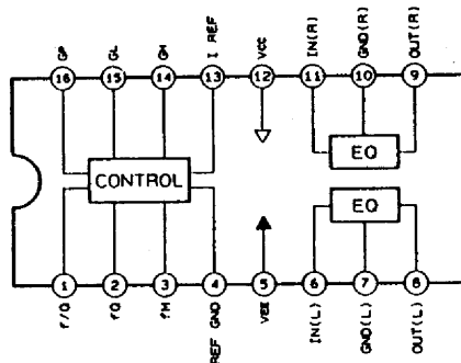
IC9 : CXA1198AP Recording Equalizer Amp
