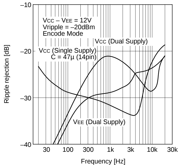
Ripple rejection
