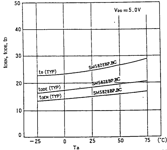
◎ t_{OEN} , t_{ODE} , t_D - T_a characteristic (Figure 3)
