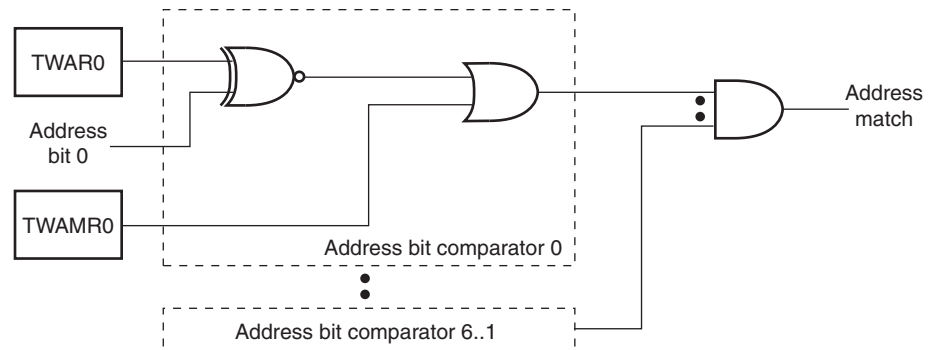
Figure 22-22. TWI address match logic, block diagram.
