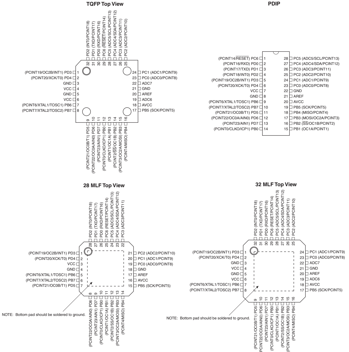
Figure 1-1. Pinout Atmel ATmega48/88/168.
