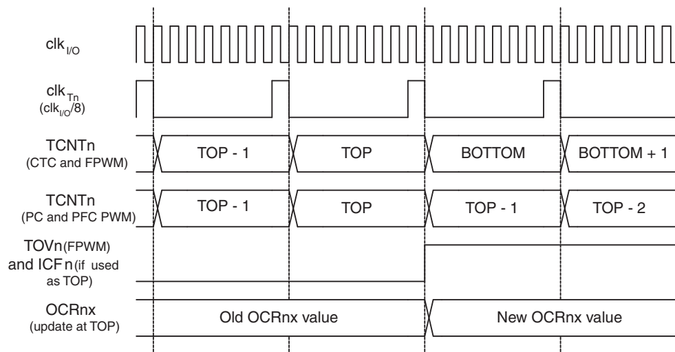
Figure 16-13. Timer/counter timing diagram, with prescaler ( f_{\text{clk\_I/O}}/8 ).
