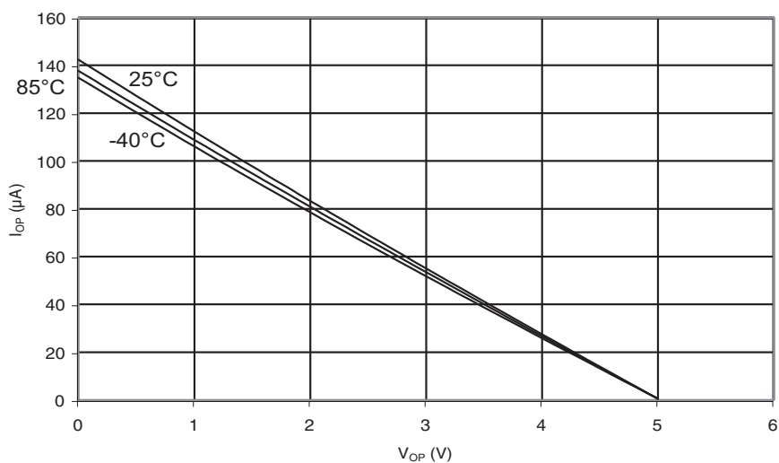
Figure 30-18. I/O pin pull-up resistor current vs. input voltage ( V_{CC} = 5V ).
