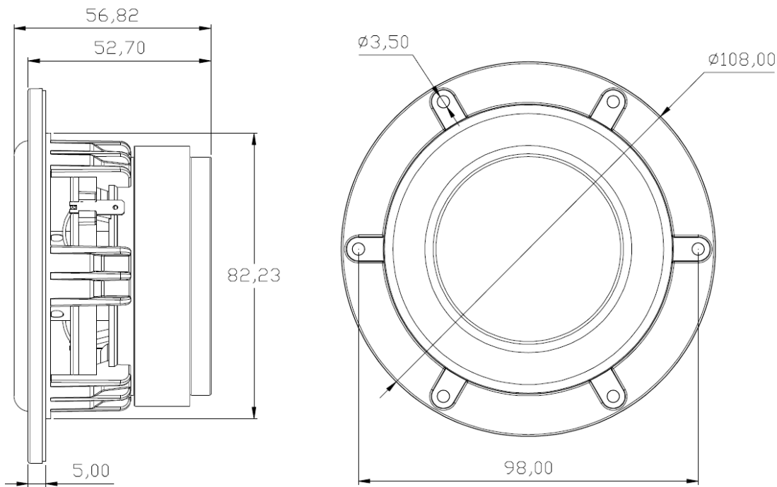
Figure 3: Nominal dimensions
