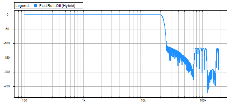
Hybrid fast roll-off filter (dB)
