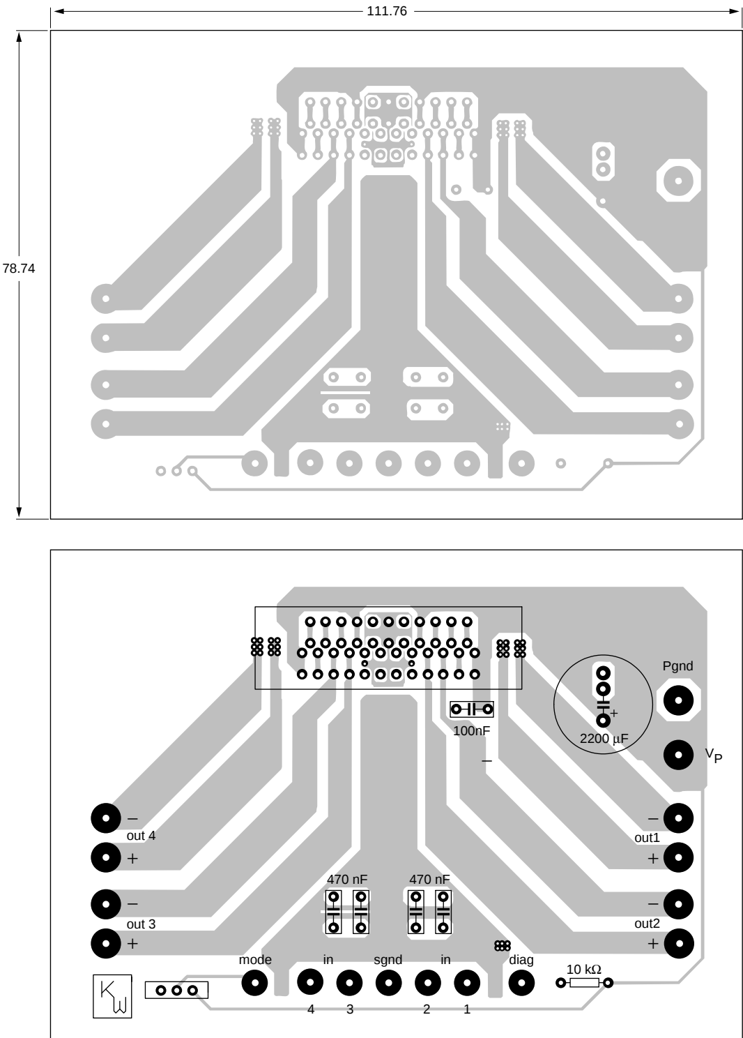
Fig.17 PCB layout (soldering side).
