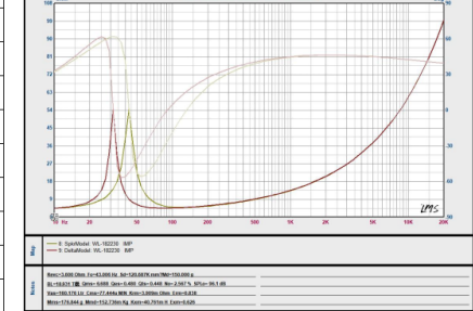
Impedance vs Freq
