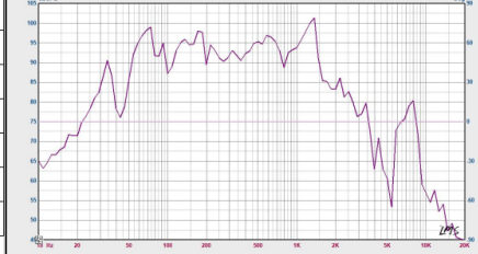
SPL vs Freq
