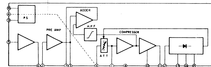
IC BLOCK DIAGRAM NE545B
