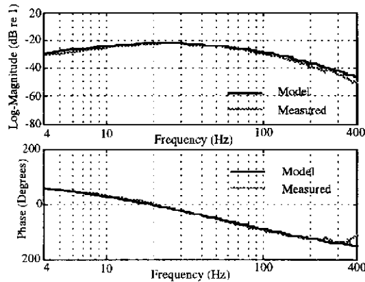
Fig. 6. Model vs. Measured Speaker Velocity Response
