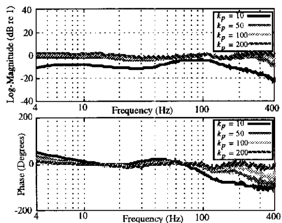
Fig. 9. Measured Closed-Loop Compensated Speaker Velocity Response vs. Proportional Gain
