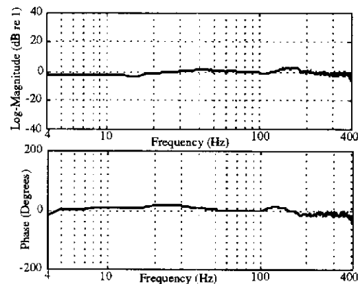
Figure 8: Compensated Secondary Speaker Coil Voltage/Laser Velocity Response
