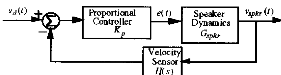
Fig. 2. Speaker Velocity Feedback Compensation Schematic
