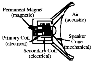
Fig. 4. Dual-Wound Coil Subwoofer Speaker Schematic
