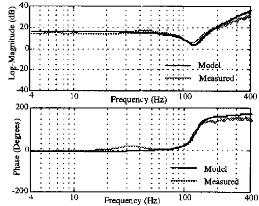
Fig. 7. Secondary Coil Voltage/Speaker Cone Velocity Model vs. Measured Responses
