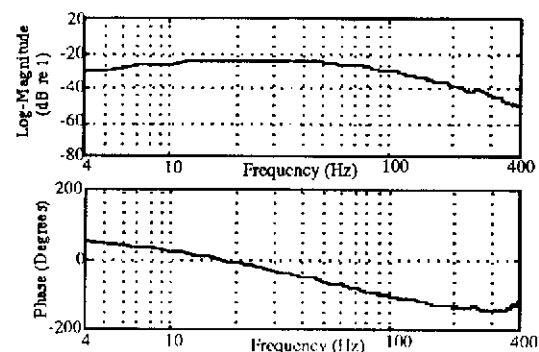
Fig. 1. Measured Velocity Response of a Typical Speaker
