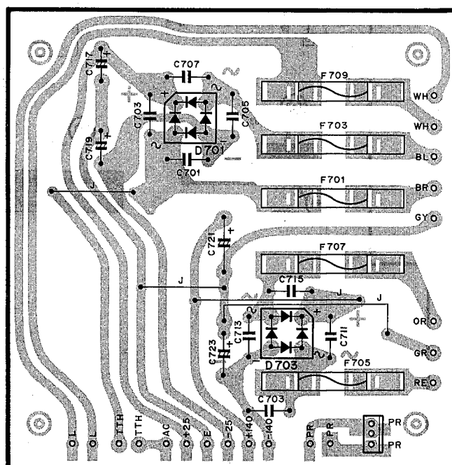
Sub Power Supply (2)
