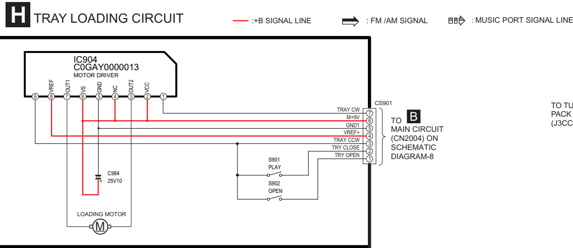
SCHEMATIC DIAGRAM-18
