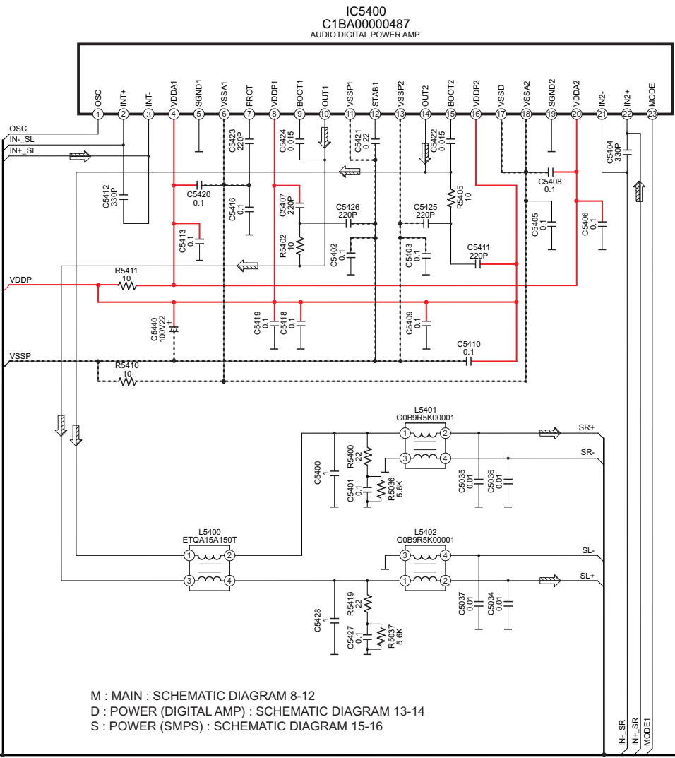
SA-HT995EE POWER(DIGITAL AMP) CIRCUIT
