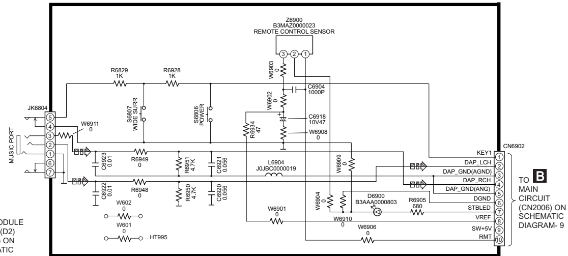
F MUSIC PORT CIRCUIT
