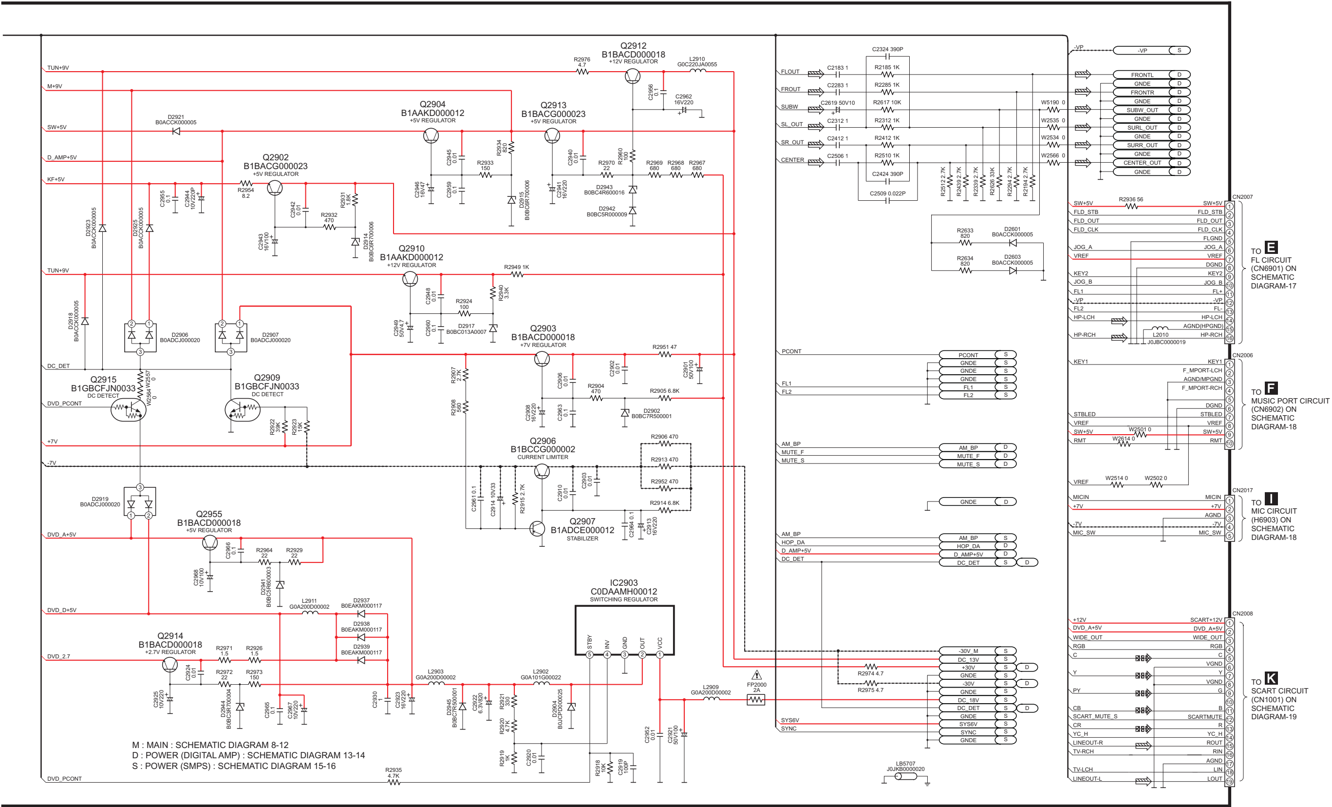
SA-HT995EE MAIN CIRCUIT
