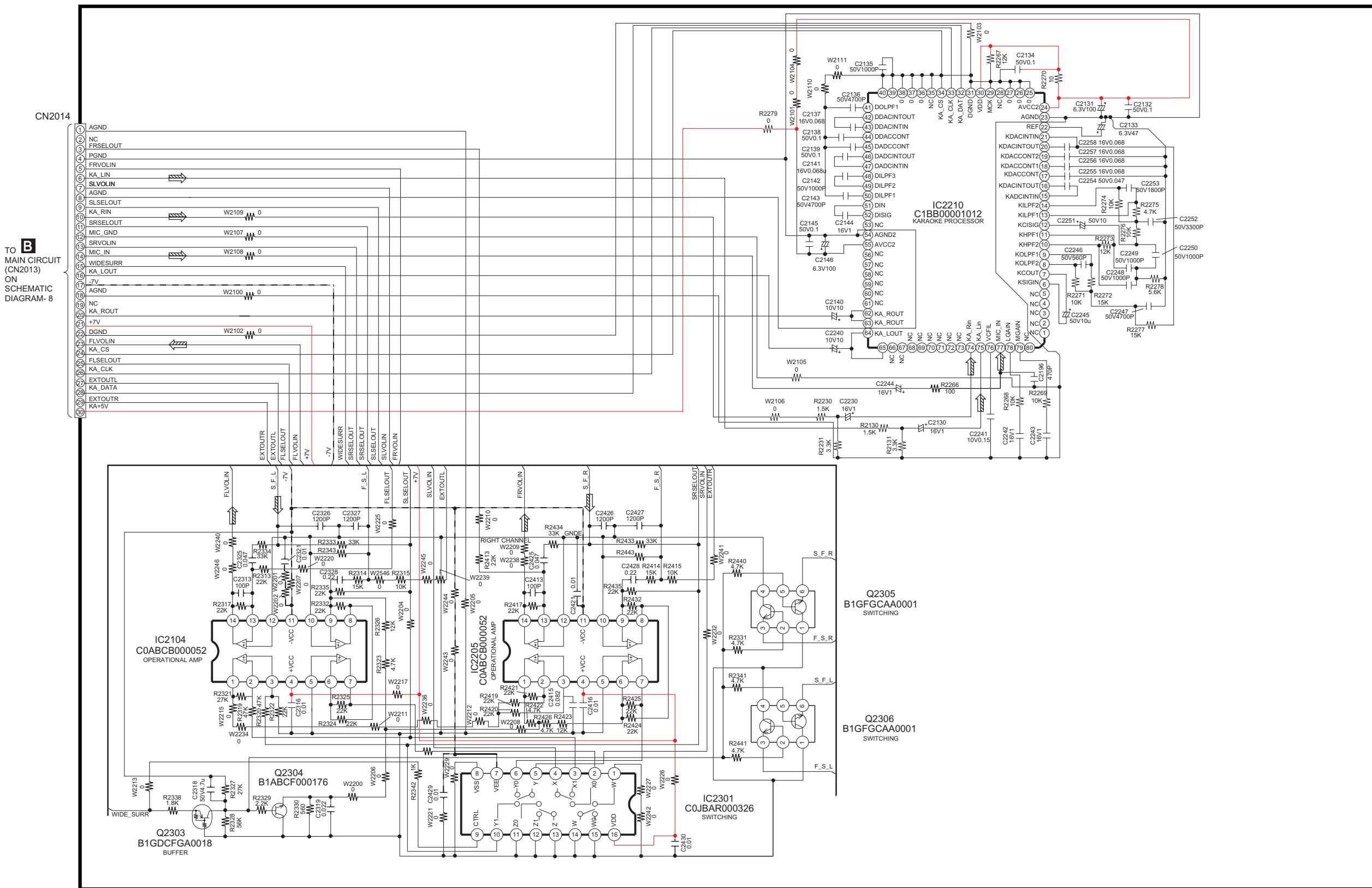
SCHEMATIC DIAGRAM-20
