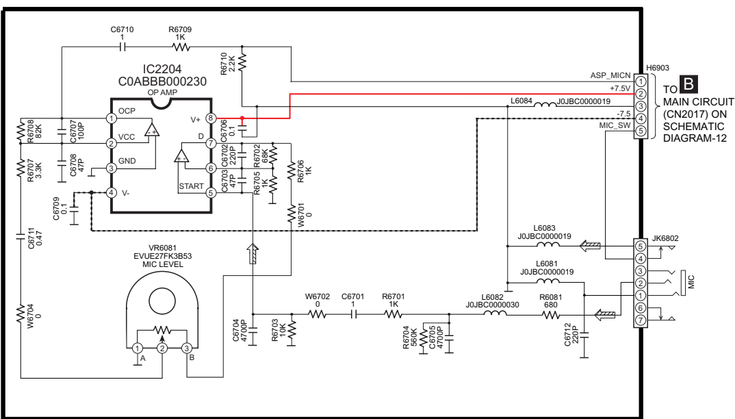
SA-HT995EE TUNER EXTENT/MUSIC PORT/TRAY LOADING/MIC/RELAY CIRCUIT
