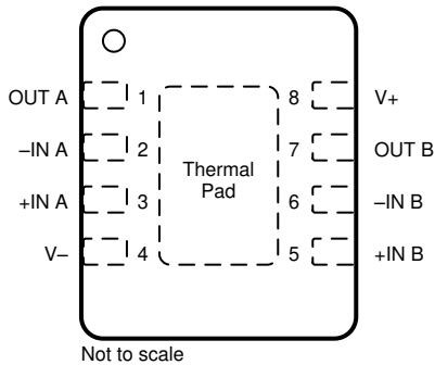
Figure 5-4. OPA1678: DRG Package, 8-Pin SON With Exposed Thermal Pad (Top View)
