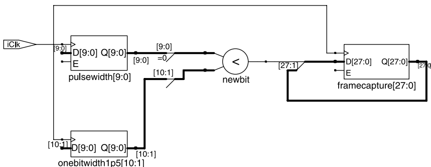
Figure 7.12 Bit detection.
