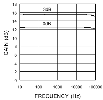
Fig.22 Center Mixing - Frequency (BD3818KS)
