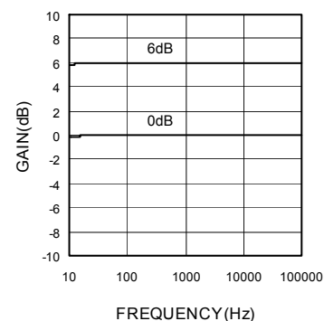
Fig.16 Input Gain - Frequency (BD3811K1)
