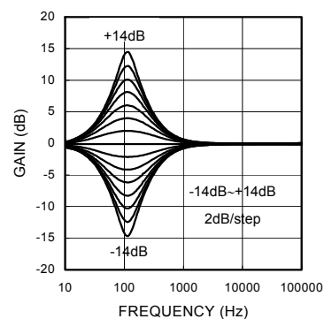
Fig.19 Bass Gain - Frequency
