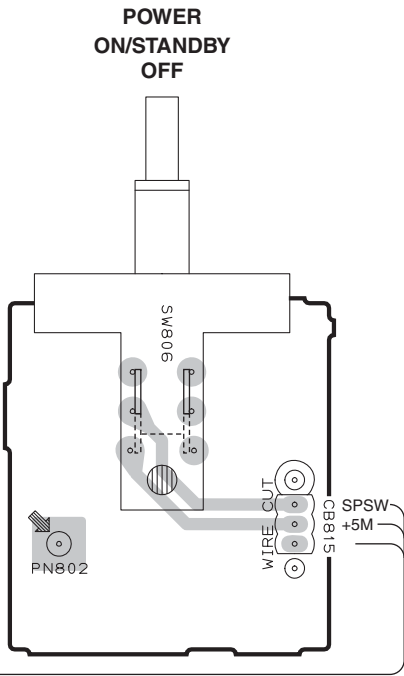
OPERATION (7) P.C.B. (Side A)
