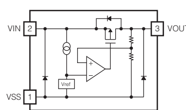
IC601: S-812C55AY-T-G Voltage regulator
