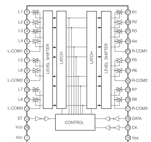
IC501: NJU7313AM Analog function switch
