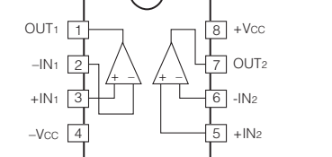
IC505-508: NJM2068MD-TE2 Dual operational amplifier
