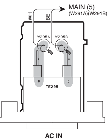
MAIN (8) P.C.B. (Side A)
