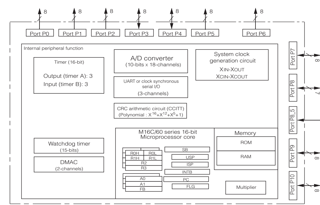
IC602: M30302MAP-A95FP Single-chip 16-bit CMOS microprocessor
