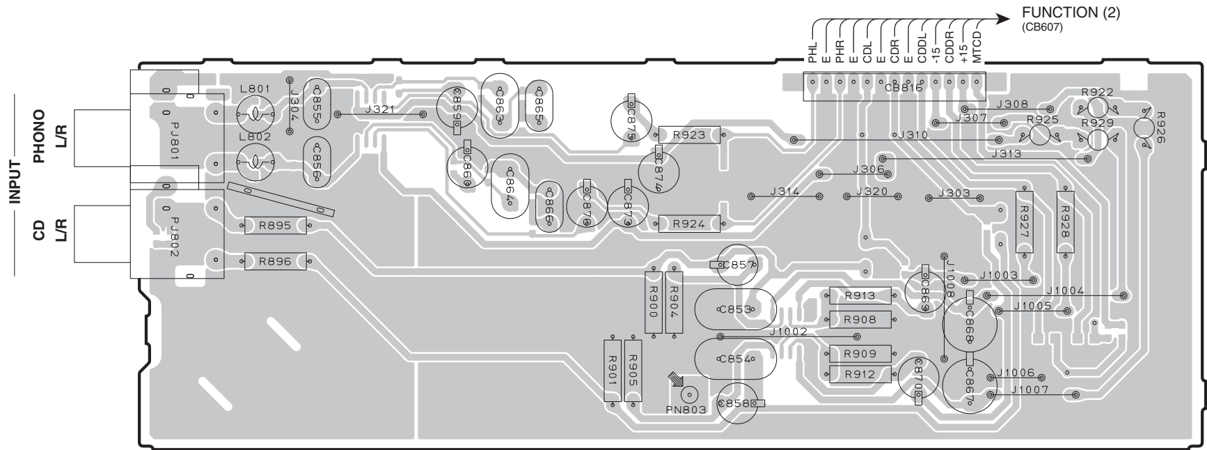
OPERATION (10) P.C.B. (Side A)
