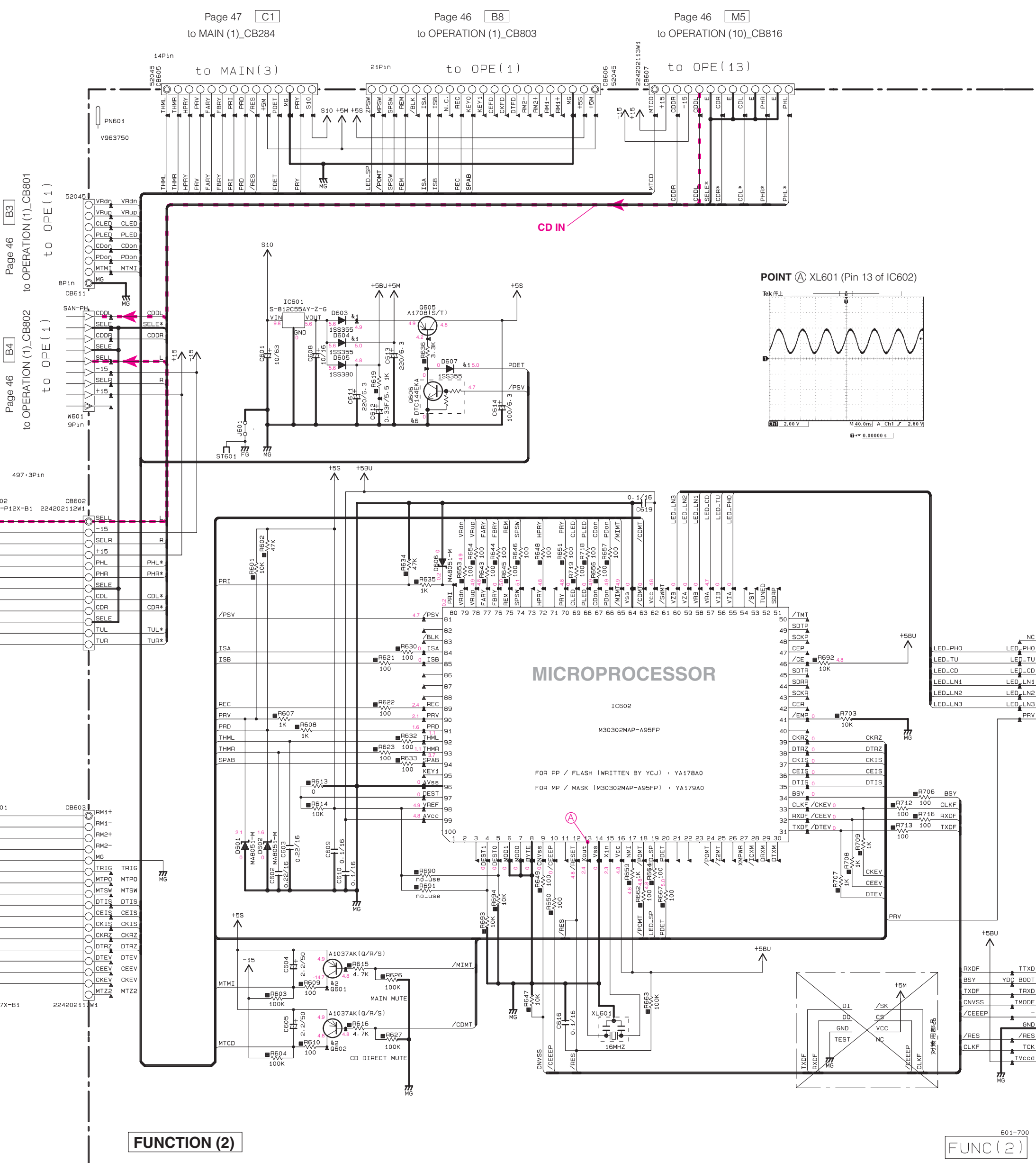
IC602: M30302MAP-A95FP Single-chip 16-bit CMOS microprocessor
