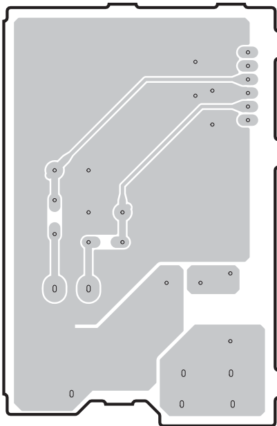
OPERATION (8) P.C.B. (Side B)
