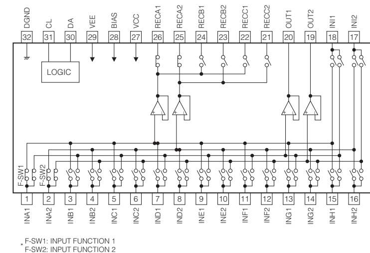
IC502: BD3841F Function switch
