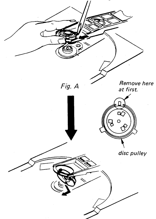
Fig. A Lift up chucking arm by hand in the direction of arrow.
