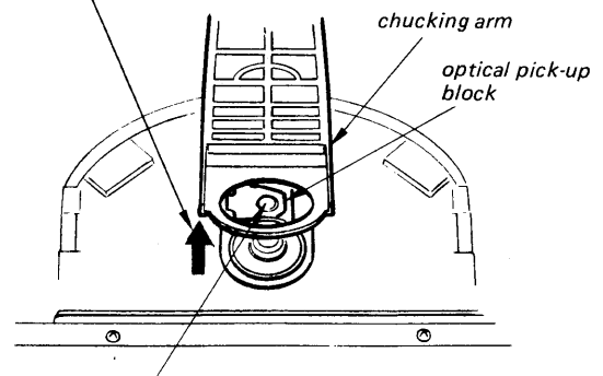
Fig. A Lift up chucking arm by hand in the direction of arrow.
