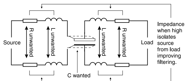
Figure 2: T-Network Capacitor
