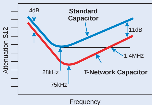
Figure 4: TNC Load Attenuation
