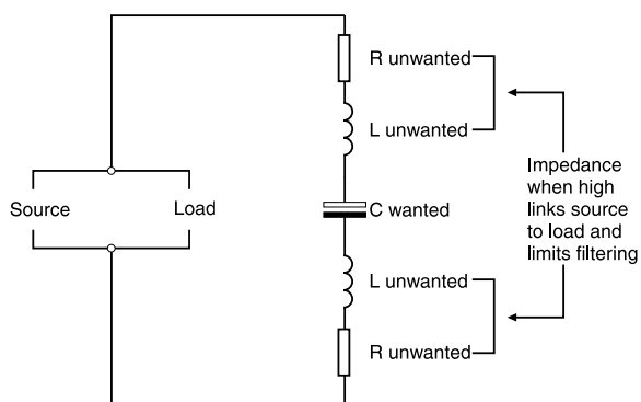
Figure 1: Conventional capacitor
