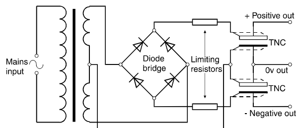
Figure 3: TNC in the Bridge Rectifier
