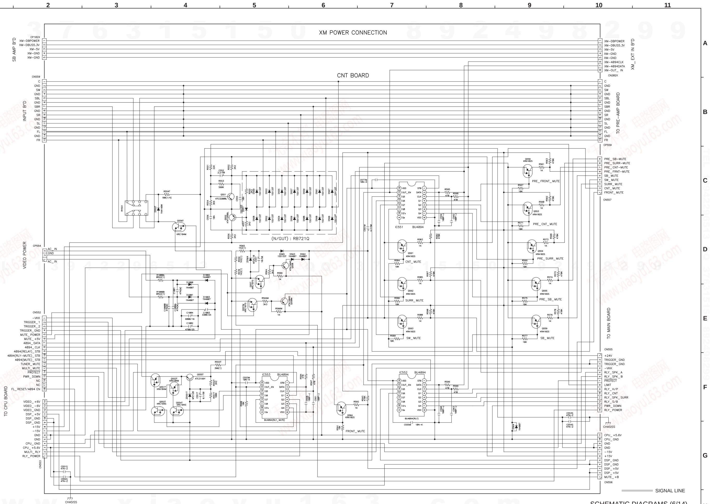
SCHEMATIC DIAGRAMS (6/14) CNT UNIT
