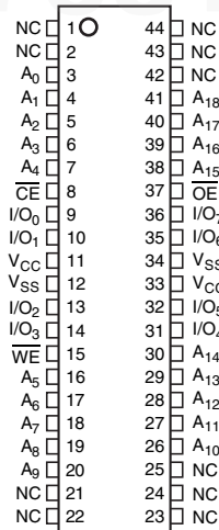
Top View
