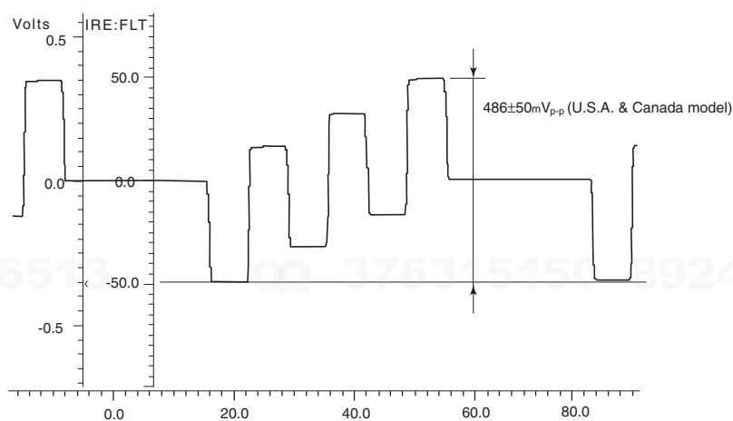
Fig.2 Cb signal
