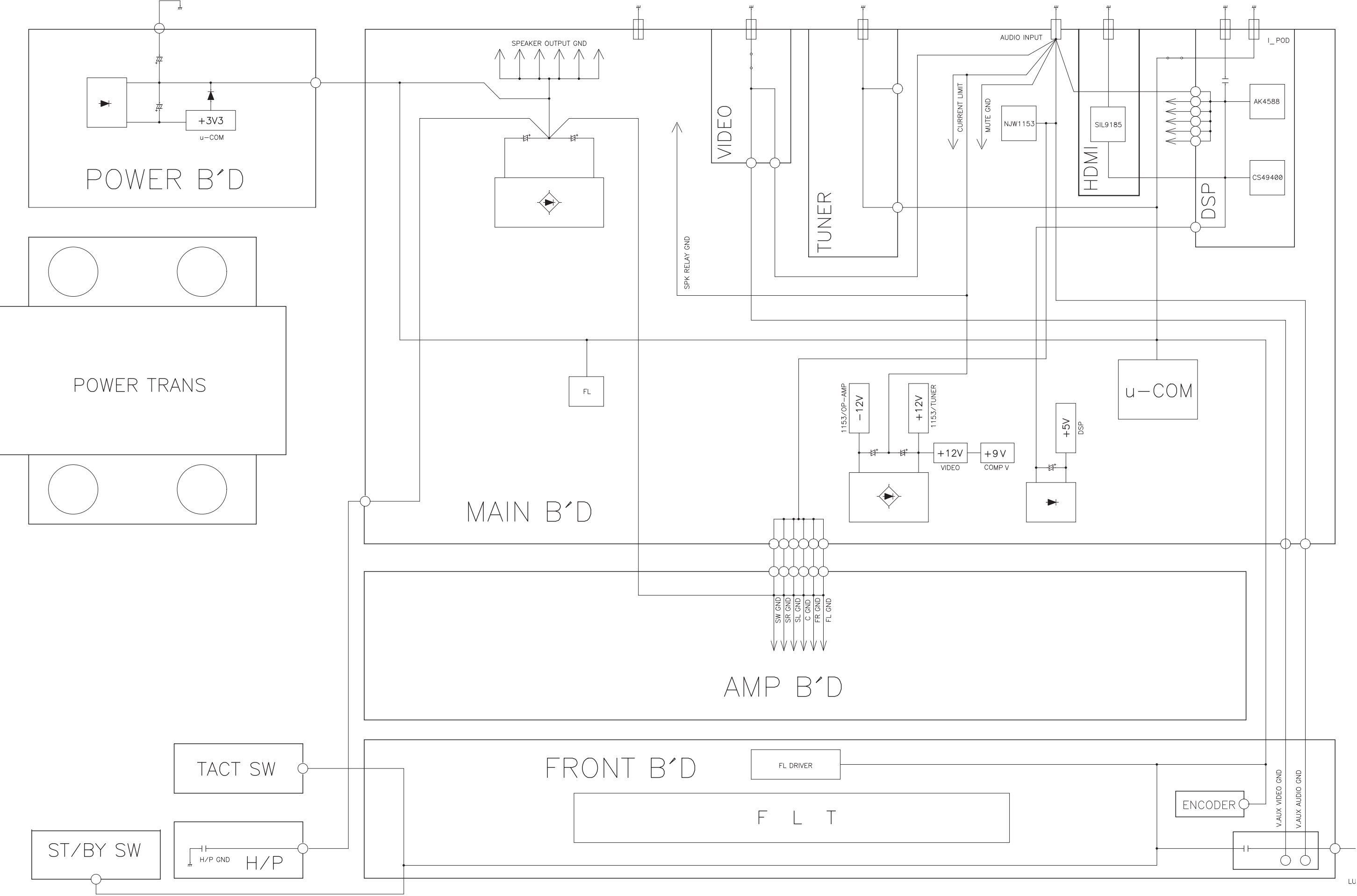
AVR-390 GND BLOCK DIAGRAM
