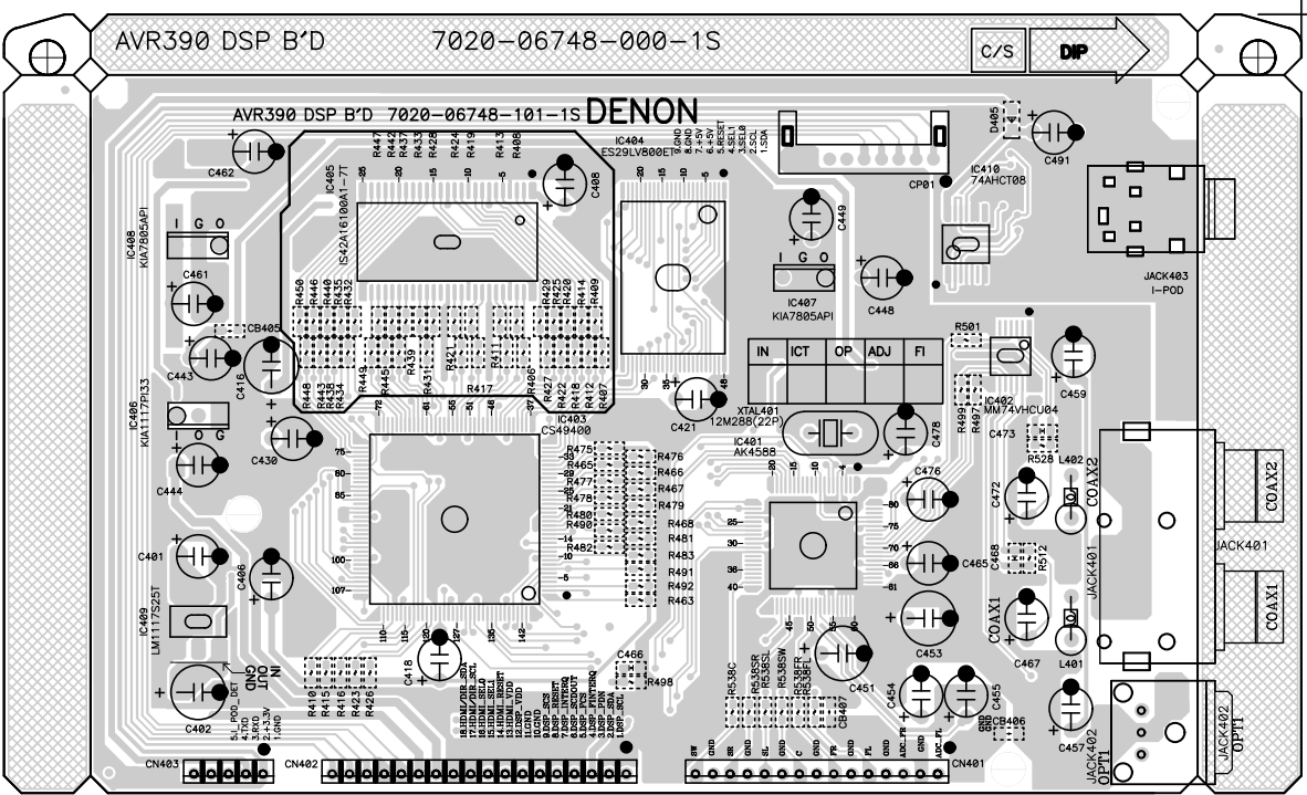
COMPONENT SIDE
