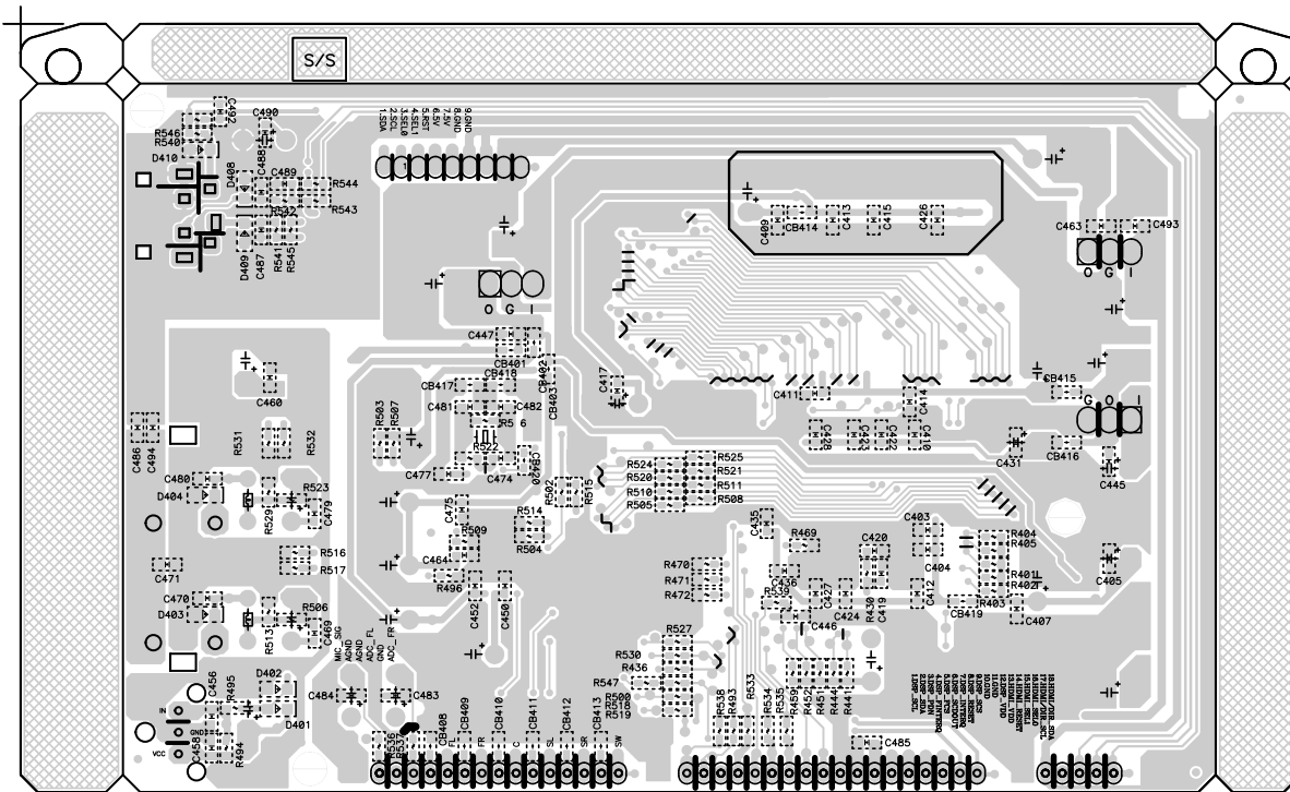
FOIL SIDE
