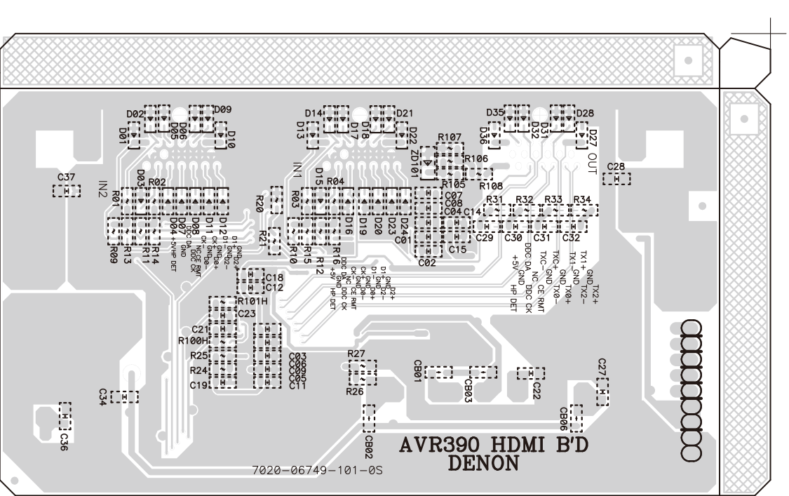
FOIL SIDE
