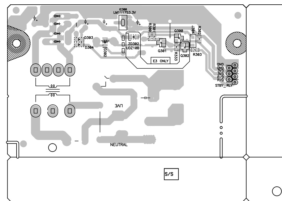
FOIL SIDE
