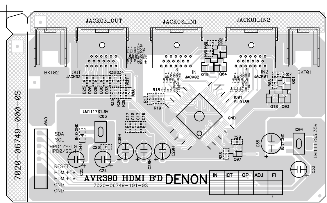
COMPONENT SIDE
