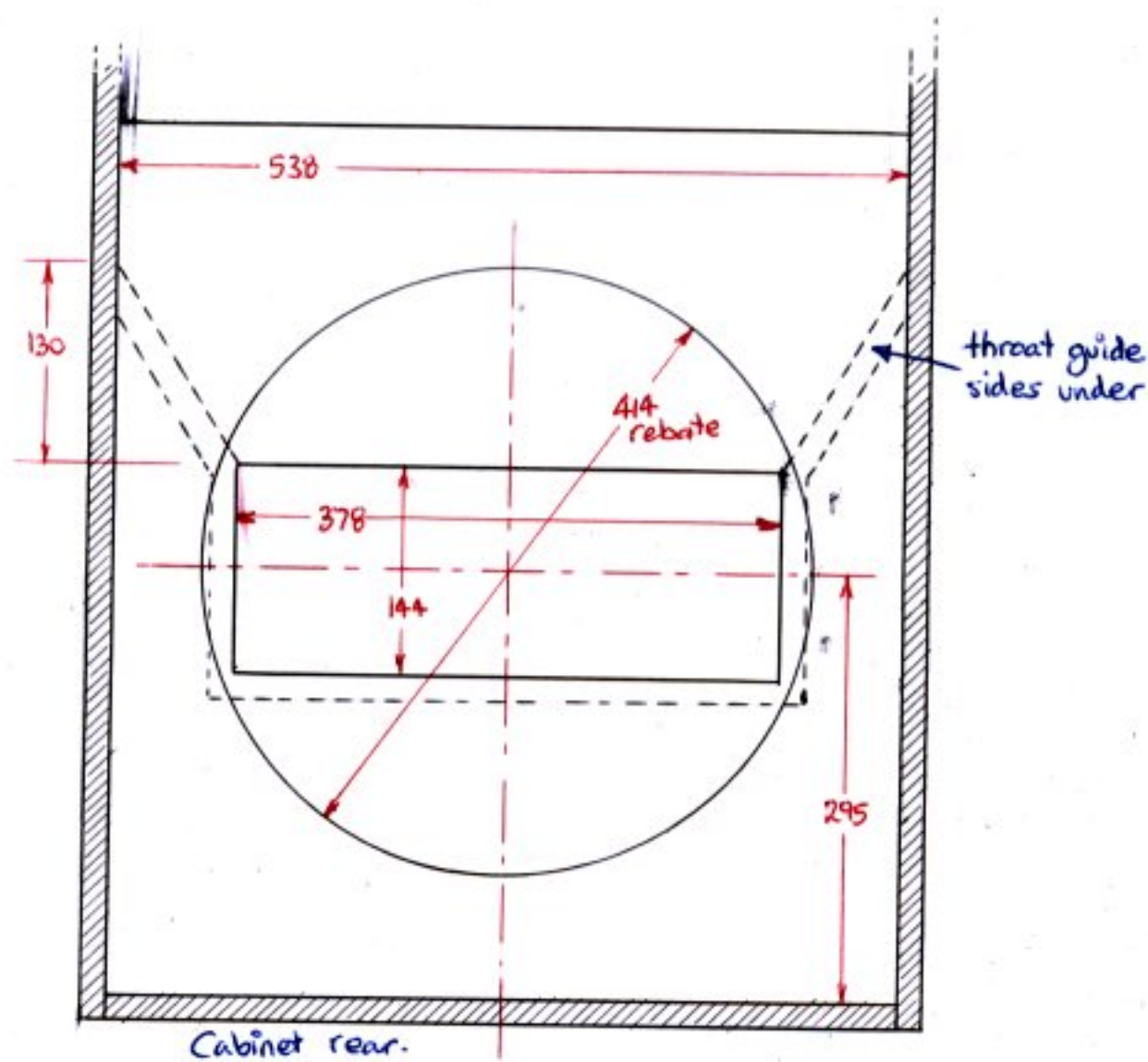
View of speaker mounting area
