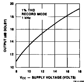
Maximum Signal Handling vs Supply Voltage
