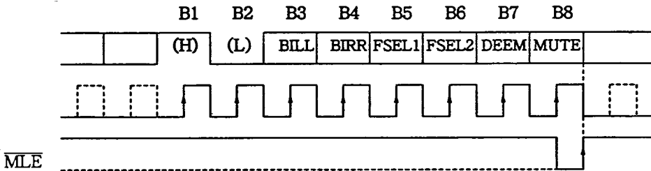
Fig. 17 Mode flag Timing 1
