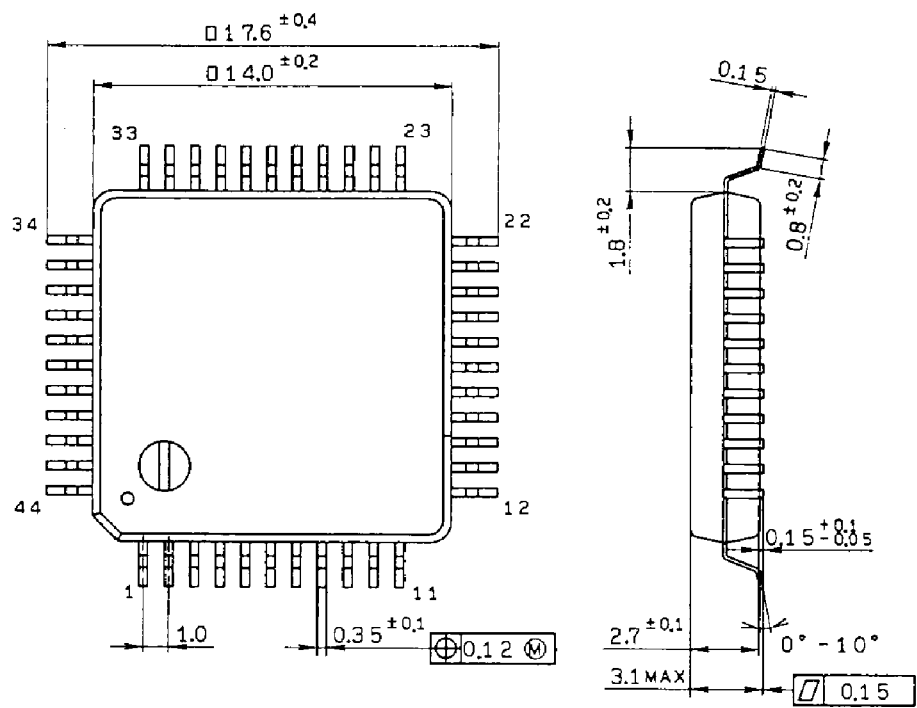
44pin QFP (Plastic) 1.1g
