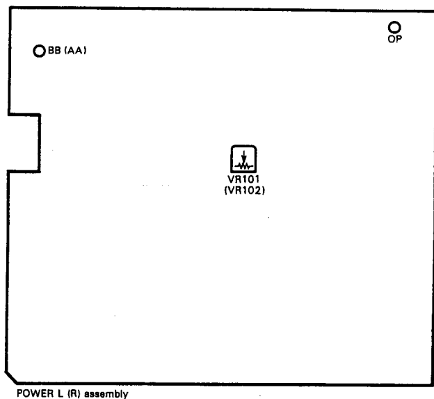
Fig. 1 Adjustment point
