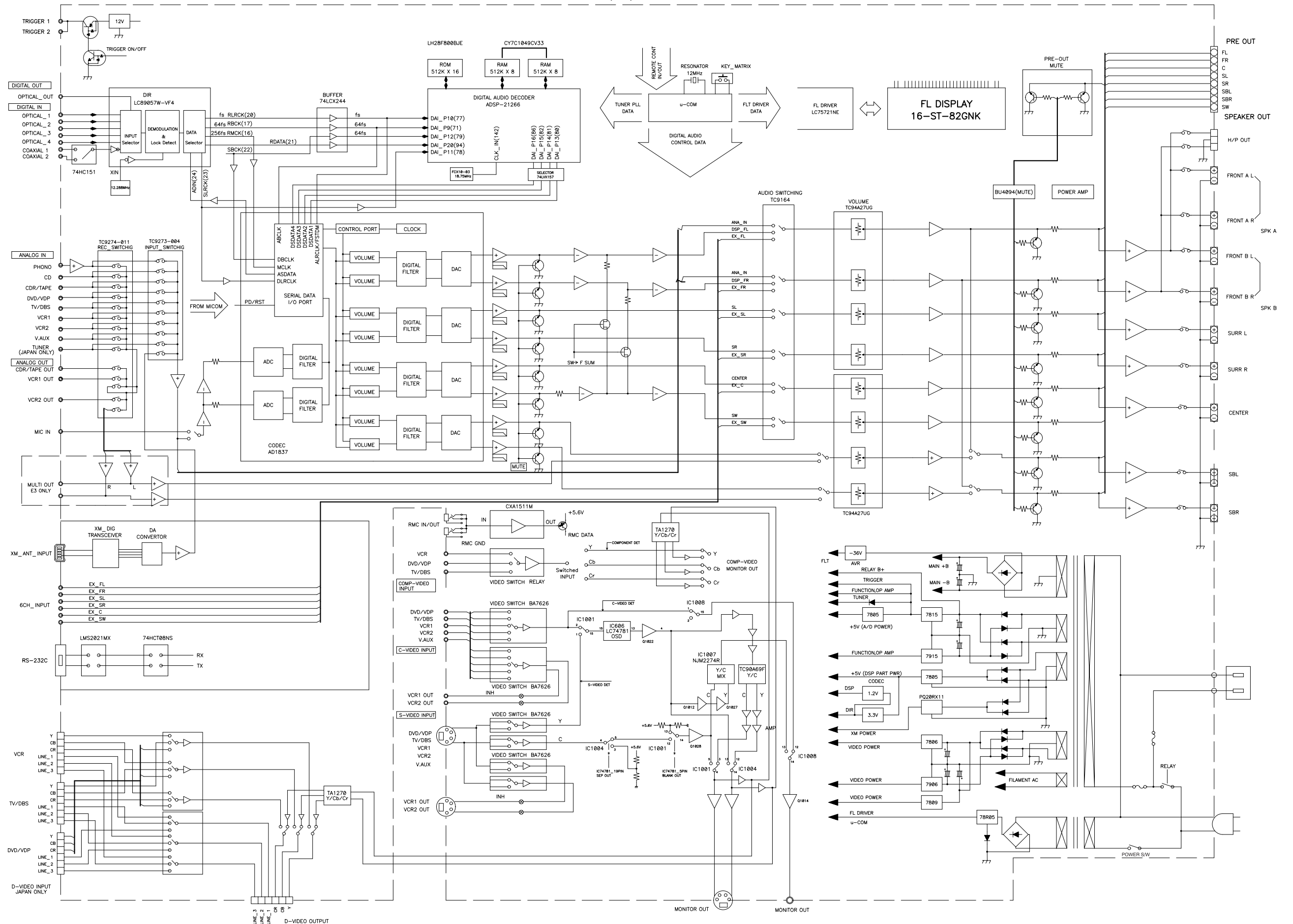
AVR 2106(E3) BLOCK DIAGRAM
