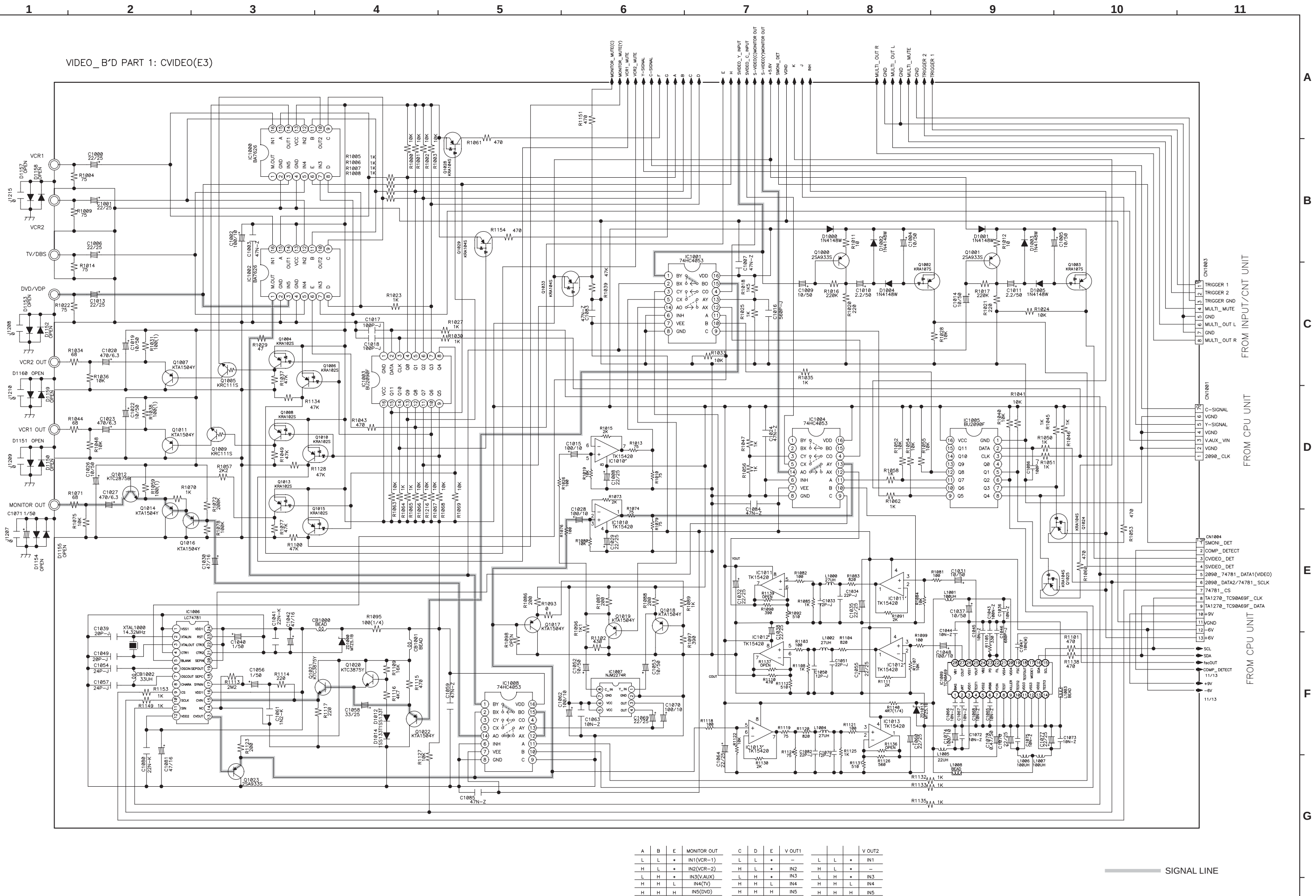
SCHEMATIC DIAGRAMS (9/14) C-VIDEO UNIT H
