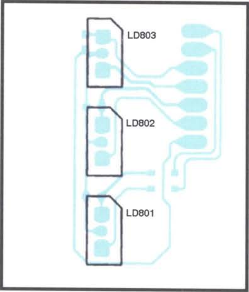
LED P.W.Board (Component Side View)
