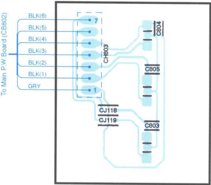
LED P.W.Board (Foil Side View)
