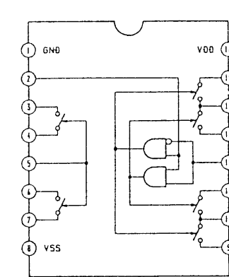
IC103, 104, 105 TC9215P
