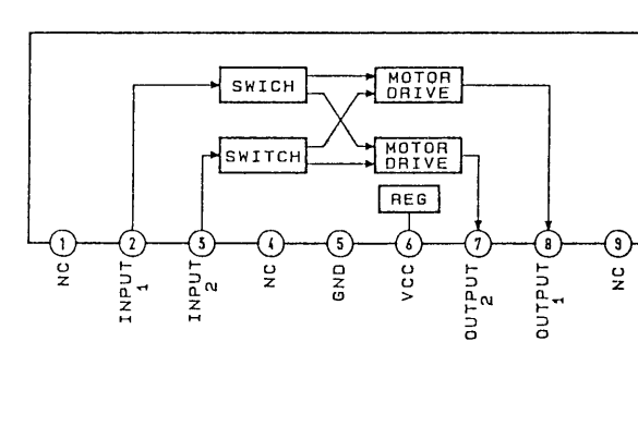
IC401 BA6208
