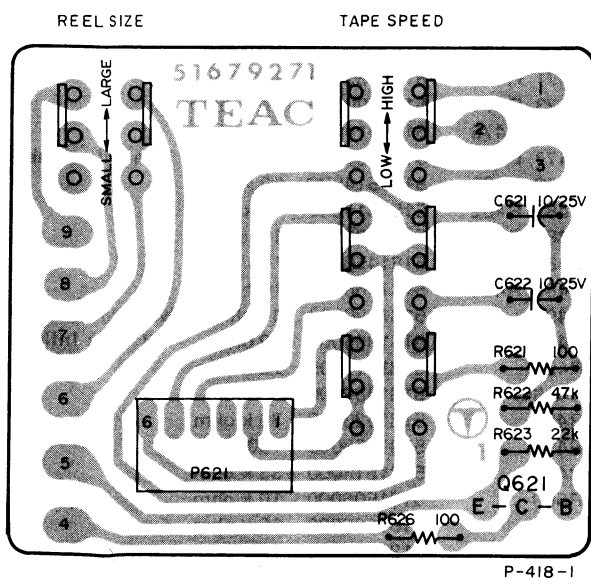
SPEED SW PCB ASSY
