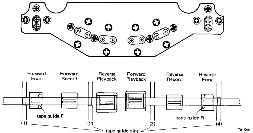
Fig. 2-17 Head arrangement
