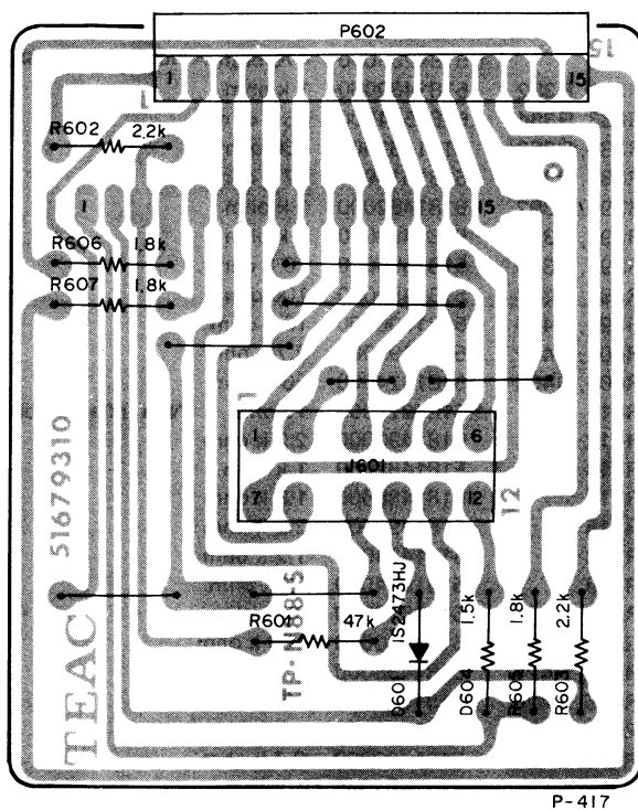
CONNECTOR PCB ASSY (X-10R)
