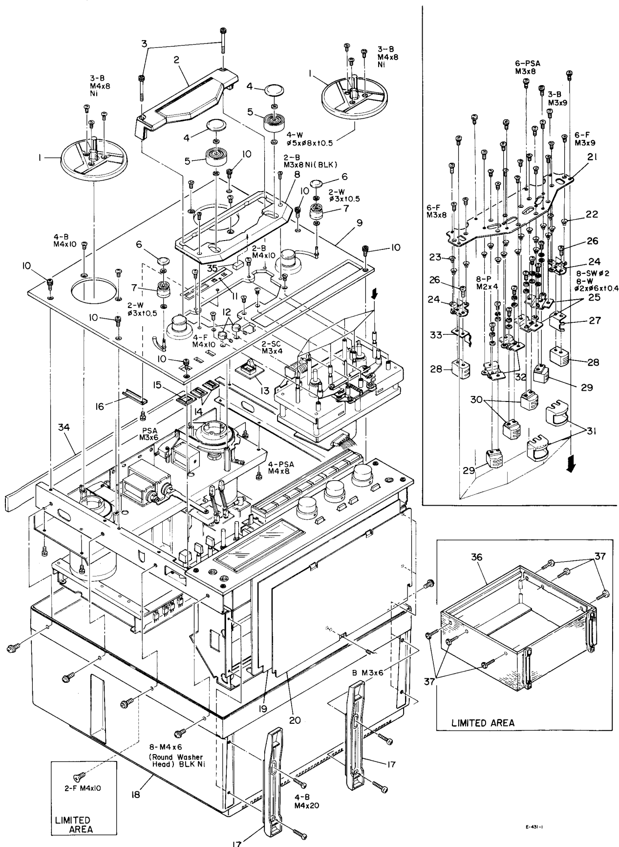
EXPLODED VIEW-1 (X10-R)
