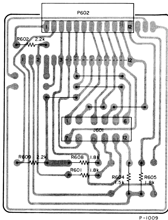
CONNECTOR PCB ASSY (X-10)
