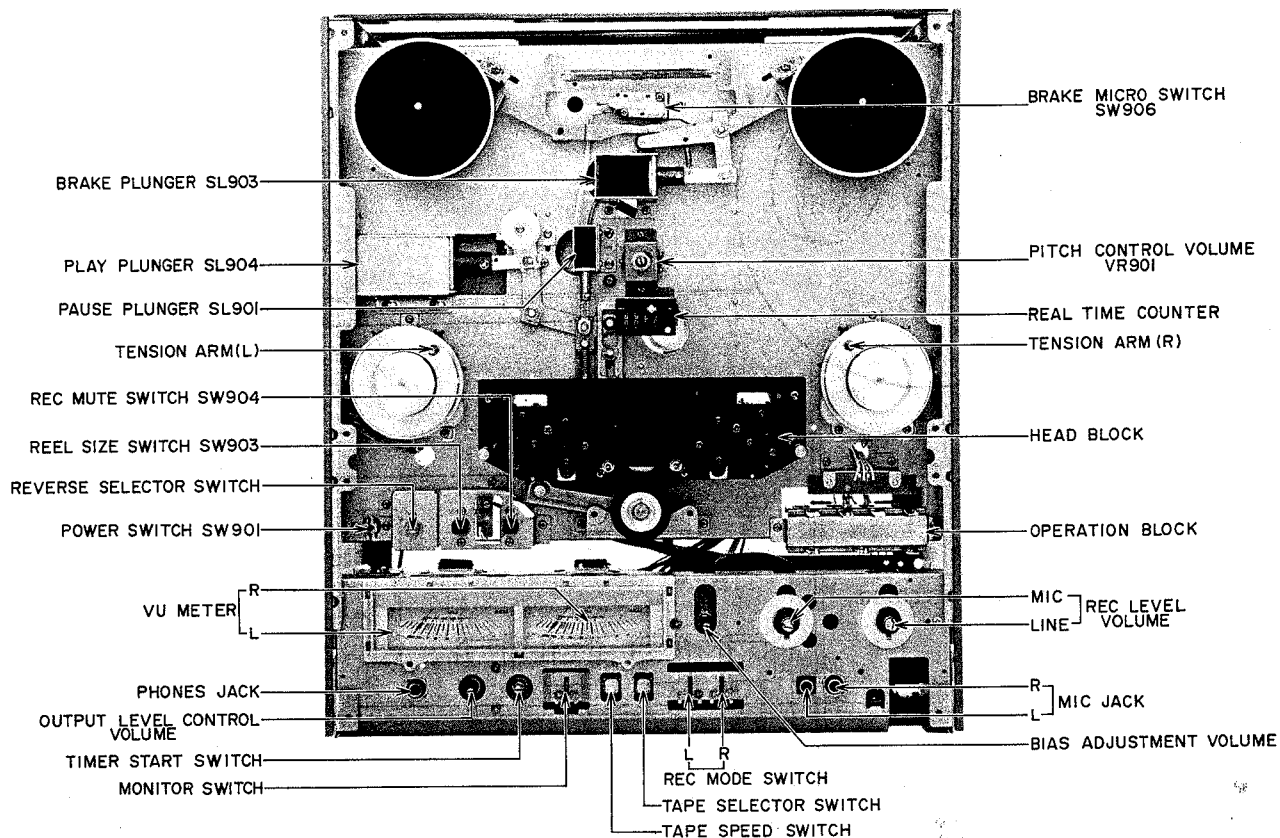
Fig. 2 Front View
