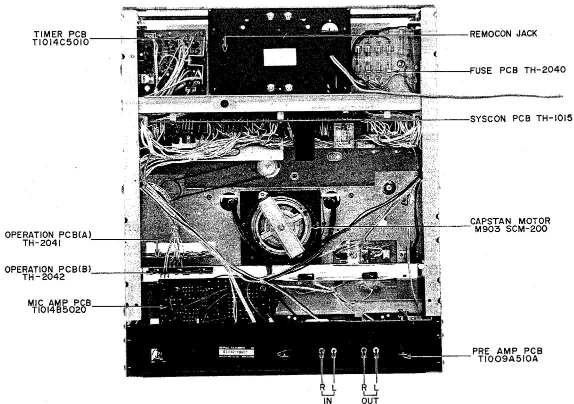
Fig. 3 Rear View
