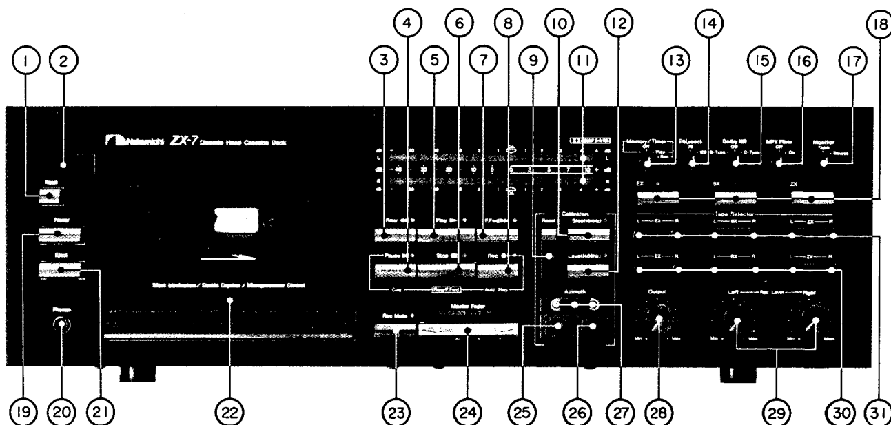
Fig. 1.1 Front View
