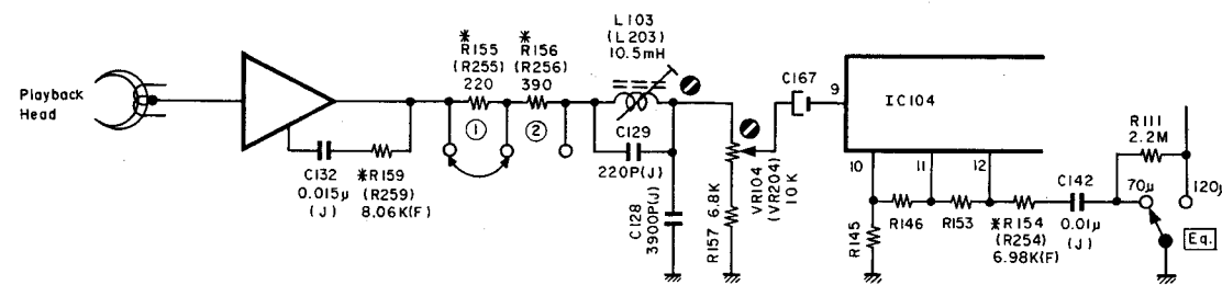
Fig. 6.12 Playback Eq. Amp.
