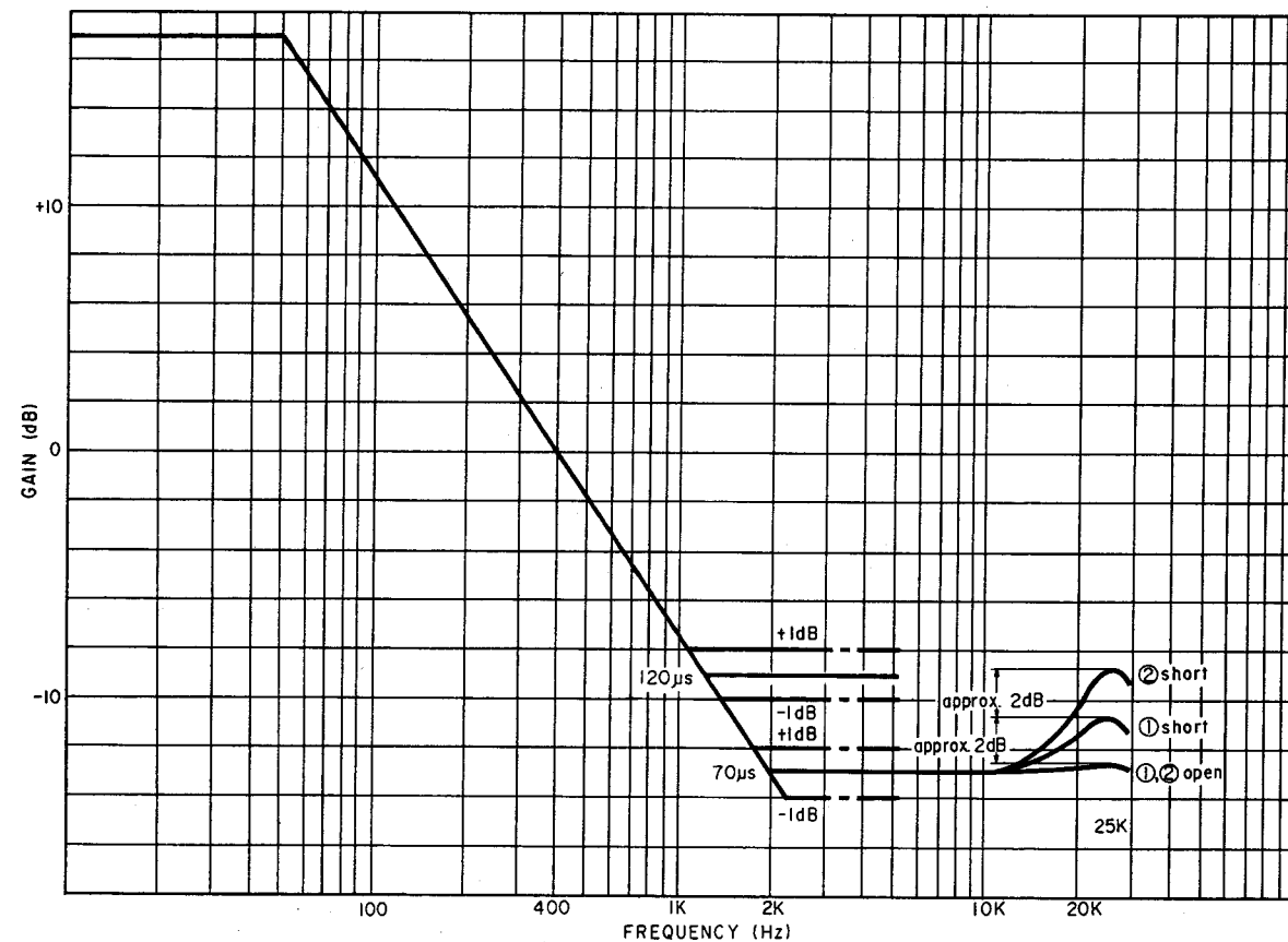
Fig. 6.11 Playback Equalization Curve
