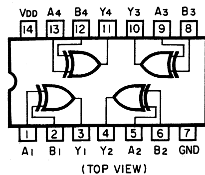
Fig. 13.9 Exclusive OR Gate C-MOS IC μPD4030BC
