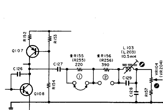
Fig. 6.5 7. Playback Level 8. Playback Frequency Response 12. Bias Trap (Playback Amp.)
