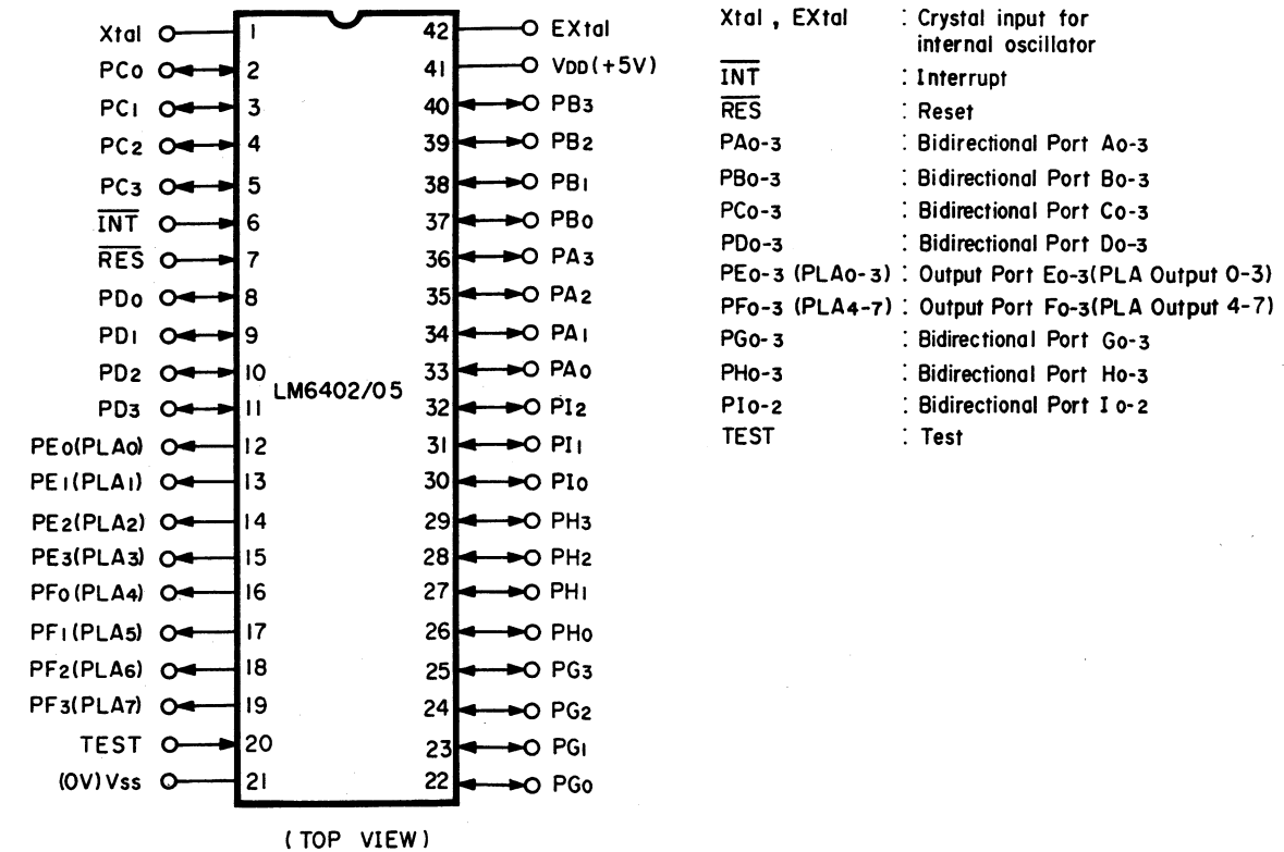
Fig. 13.12 4-Bit Micro-processor LM6402A-052/048
