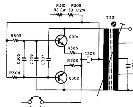
Fig. 6.6 9. Bias Oscillation Frequency and Erase Current
