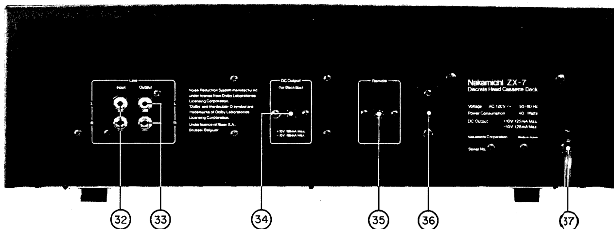
Fig. 1.2 Rear View
