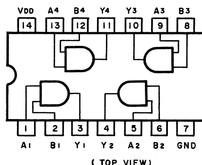
Fig. 13.8 AND Gate C-MOS IC \mu PD4081BC
