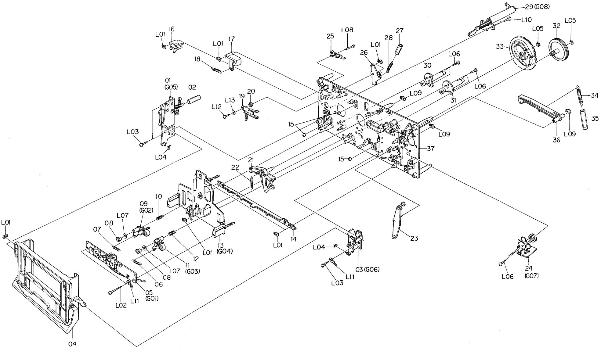
8.12. Main Mechanism Chassis Ass'y (D03)
