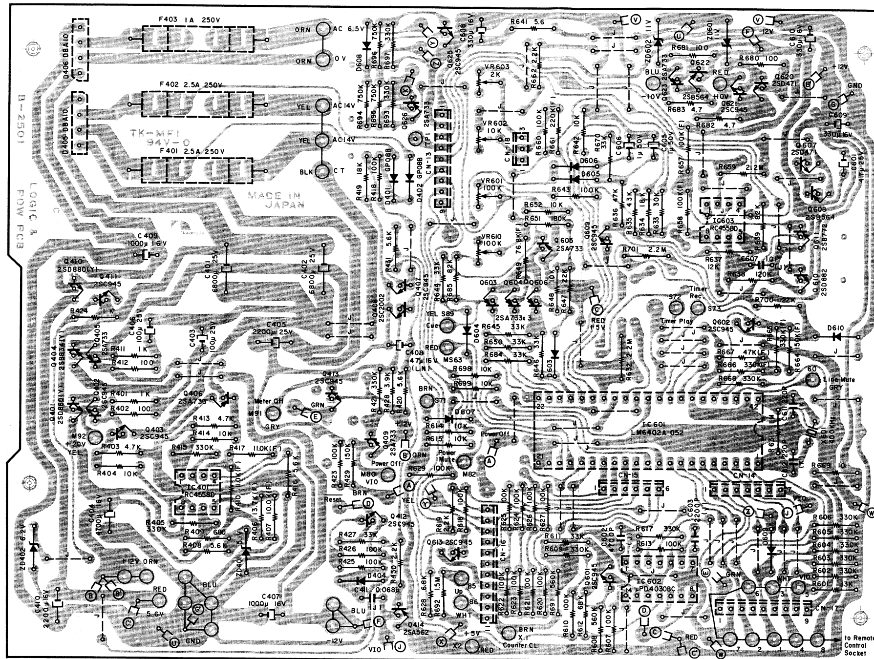
Fig. 7.13.1 Serial No.: A12402301 -
