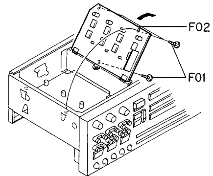
(A) Bottom View
