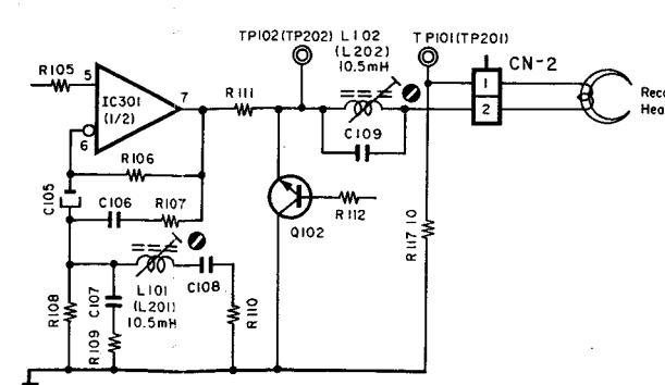
Fig. 6.7 10. Record Amp. Equalizer 11. Bias Trap (Record Amp.)
