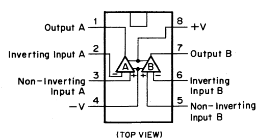
Fig. 13.5 Operational Amp. IC RC4558D, RC4558DD, \mu PC4556C, RC4560D, RC4559D, TA75558P-R
