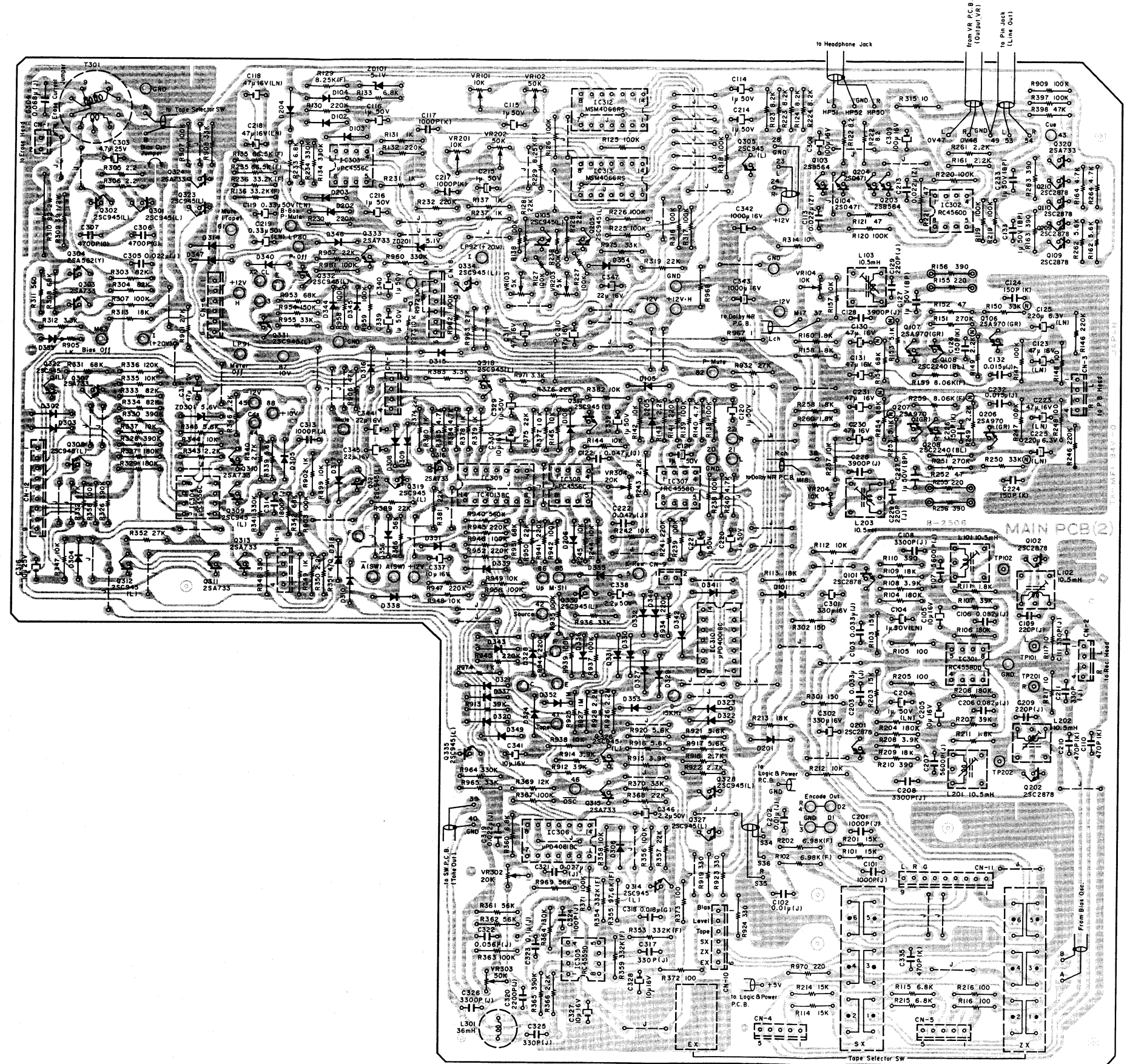
Fig. 7.14.2 Serial Nos.: A12403401 - A12404900 Note: Diode is 1S553, 1S953, or 1S1555 unless otherwise specified.
