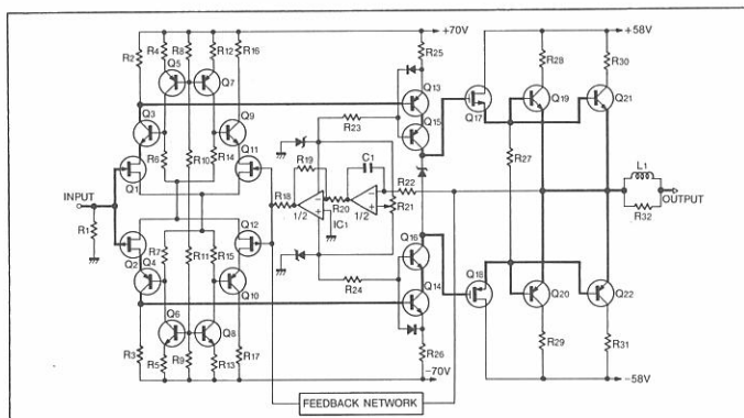
Diagram of Cascode Bootstrap connection Input stage and Parallel Push-pull Output stage
