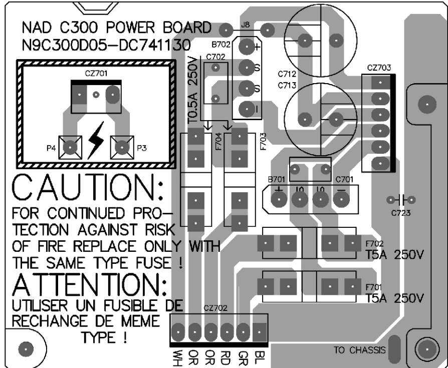
Power Board
