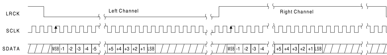
Figure 4. Format 1 - I²S up to 24-bit Data
