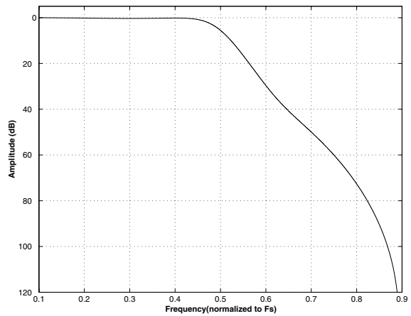
Figure 41. Quad Speed (slow) Transition Band
