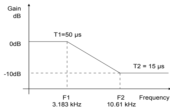
Figure 17. De-Emphasis Curve
