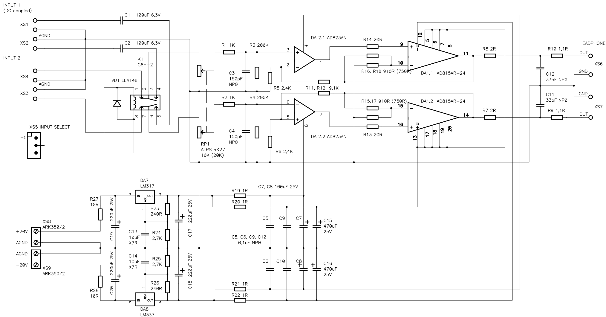
Headphone Amplifier HA1.2 schematic rev.1
