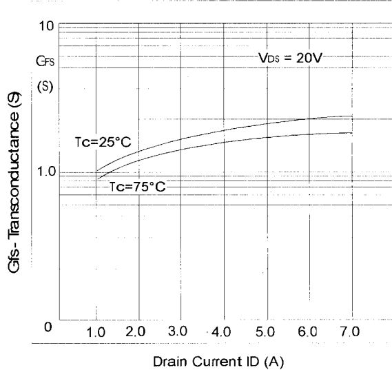
Forward Transfer Admittance (P-Channel)
