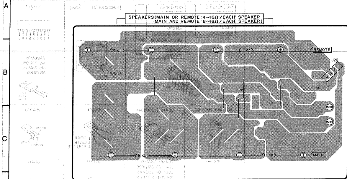
N SPEAKER TERMINAL P.C.B.
