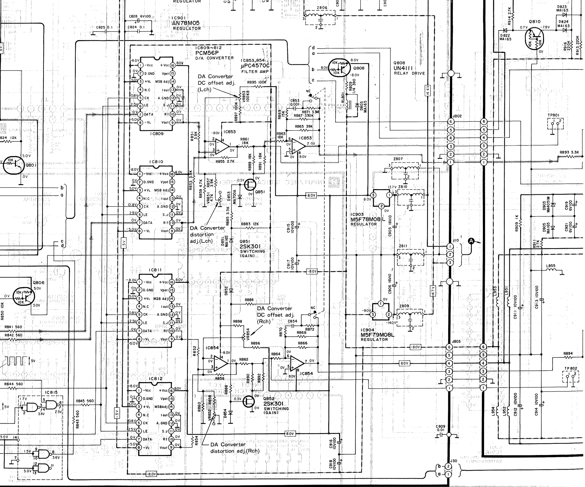
C AUDIO(DIGITAL) AMP CI
