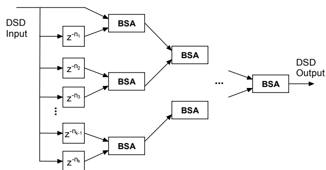
Figure 3: Implementation of a basic flanger or chorus using the bitstream adder (BSA) of Figure 2.
