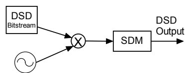
Figure 4: Modulation of a DSD bitstream.
