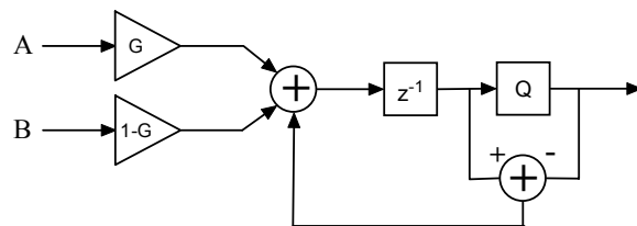
Figure 7: Smooth switching between DSD bitstreams using a slowly changing gain and a first order SDM.
