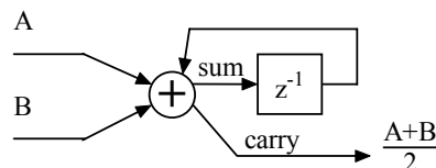
Figure 2: A bitstream adder.
