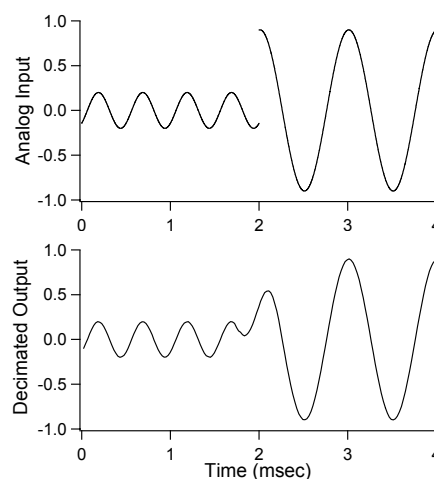
Figure 8: Smooth switching between DSD bitstreams using the circuit from Figure 7. This is the worst case scenario, where the input bitstreams have differing amplitudes and opposing phases.
