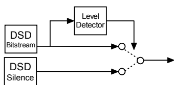
Figure 5: A hard noise gate implemented on a DSD bitstream. A DSD silence signal must be used since constant DC levels are not possible.
