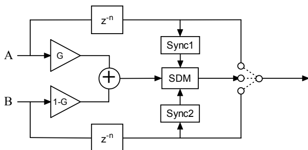
Figure 6: Smooth switching between bitstreams using synchronisation.
