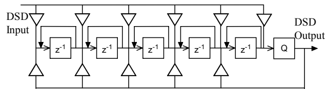
Figure 9: Configuration of a combined IIR filter and remodulator.
