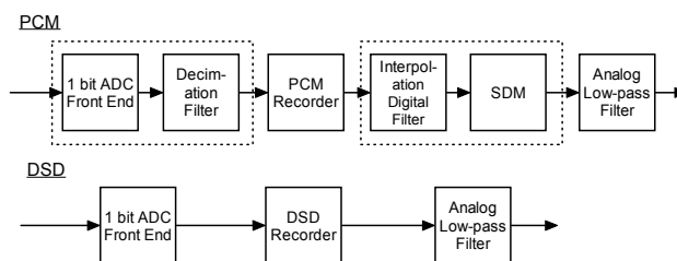
Figure 1: The standard multibit PCM recording and playback chain, (a), requires a decimation filter on the recording side and an oversampling filter on the playback side, whereas Direct Stream Digital, (b), enables sound to be recorded directly in the 1-bit signal format and eliminates the need for these filters.
