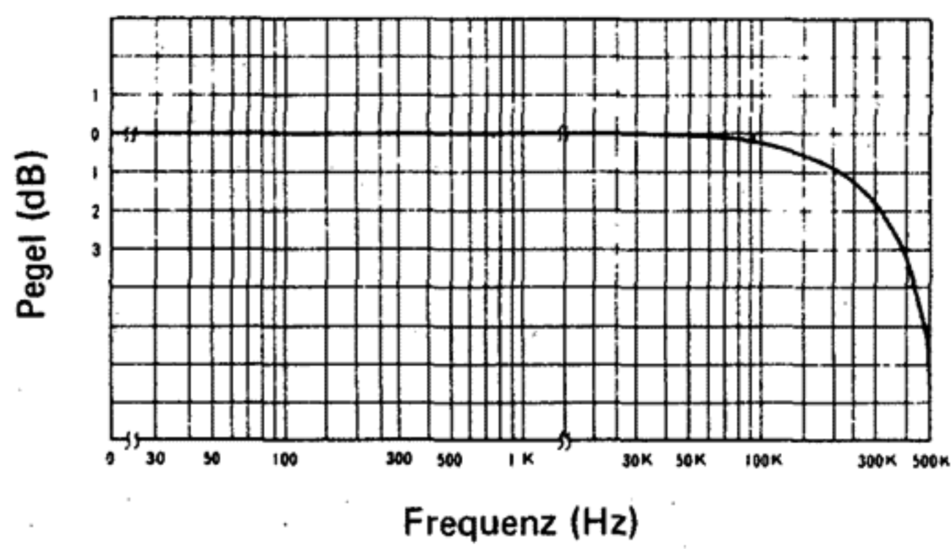
Frequenzgang
