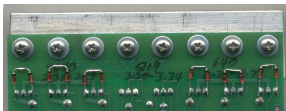
Figure 5 The protection diodes installed back-to-back between gate and source of the output MOSFETs.
