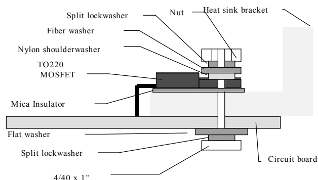
Figure 2 Mounting of metal tab TO220 power transistors.
