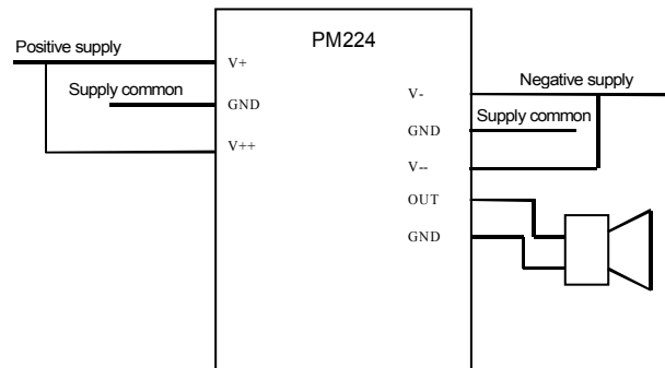
Power supply hookup
