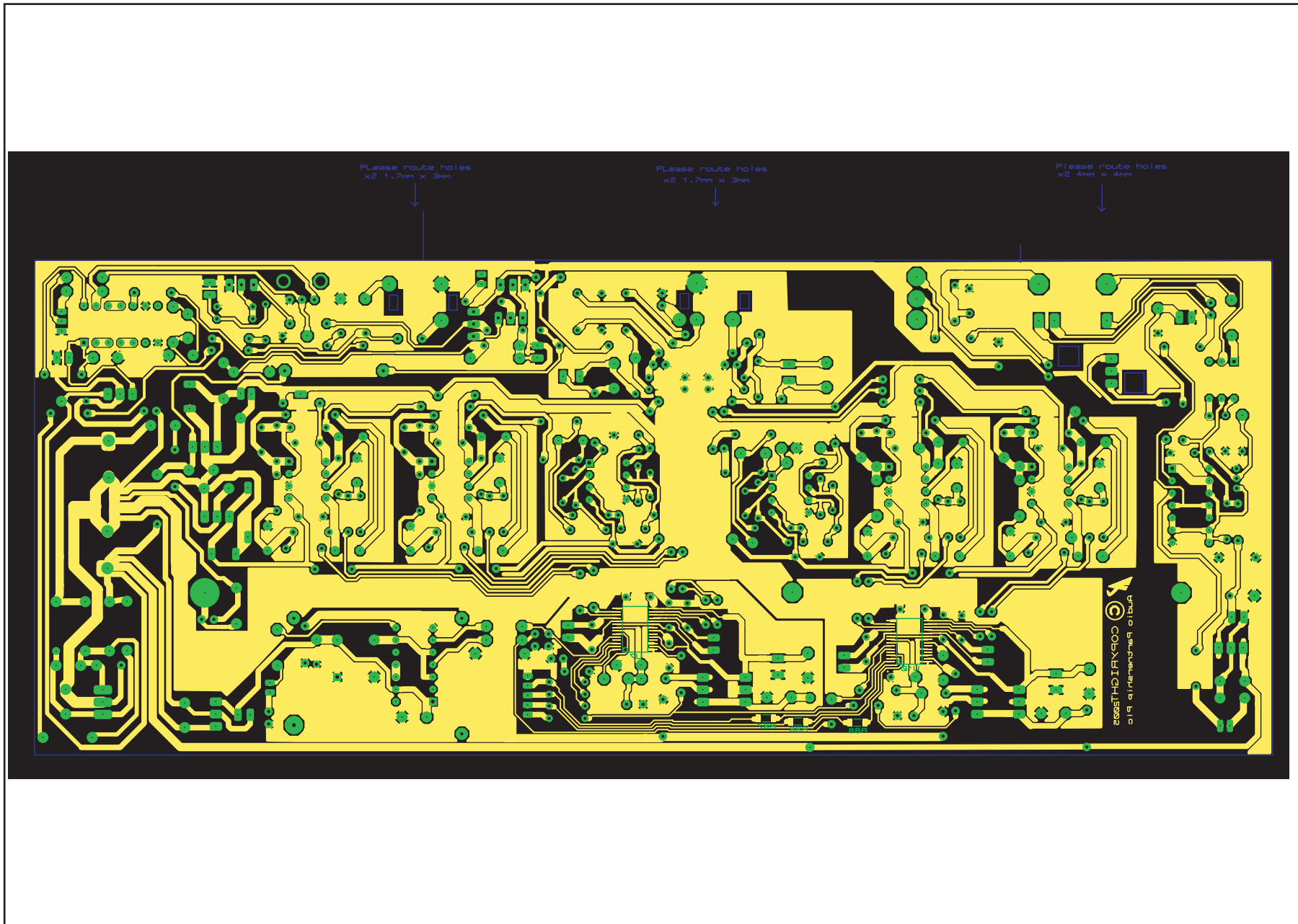
API7613/6 DAC Board PCB Layout (Bottom Side)
