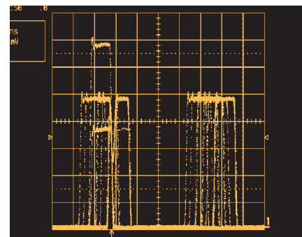
Above, Exclusion Trigger is set to eliminate pulses within a width of 50 ns. Only pulse widths that are not 50 ns wide will trigger the scope.
