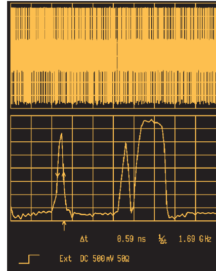
Top trace: 1 ms time window captured using 4 GS/s and 4 MBytes of record length. Bottom trace: zoomed portion showing a .59 ns pulse expanded for detailed examination.
