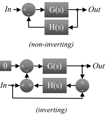
Figure 1: Block Diagram Representations of Negative-Feedback
