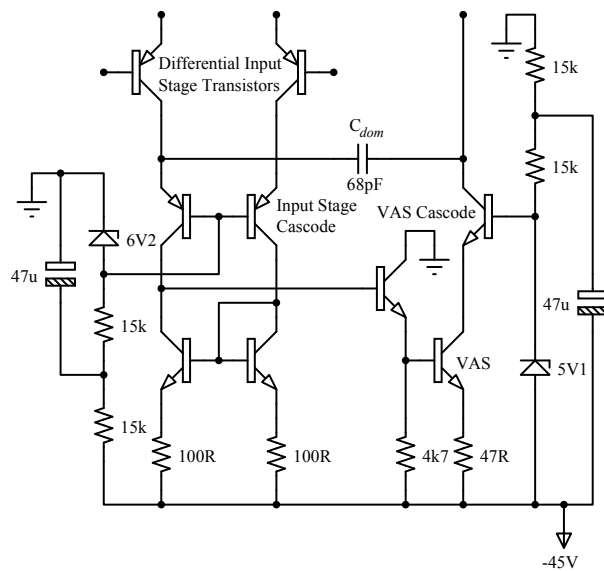
Figure 17: Cascoding in a Single-Dominant-Pole Amplifier
