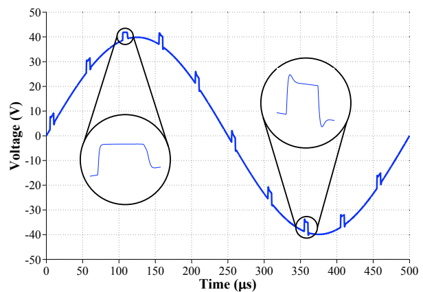
Figure 14: Results of Transient Analysis of Amplifier with Two-Pole Compensation (8 \Omega load, voltage measured at output before inductor.)
