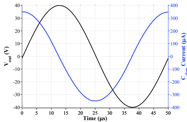
Figure 6: Current Flowing in C_{dom} with 20 kHz Amplifier Output Signal
