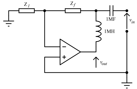
Figure 8: Observing Loop Gain in High-Gain Circuits by Modification of the Feedback Loop
