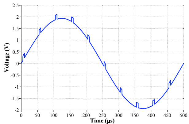
Figure 13: Amplifier Input Signal for Transient-Analysis Investigation of Stability [7]
